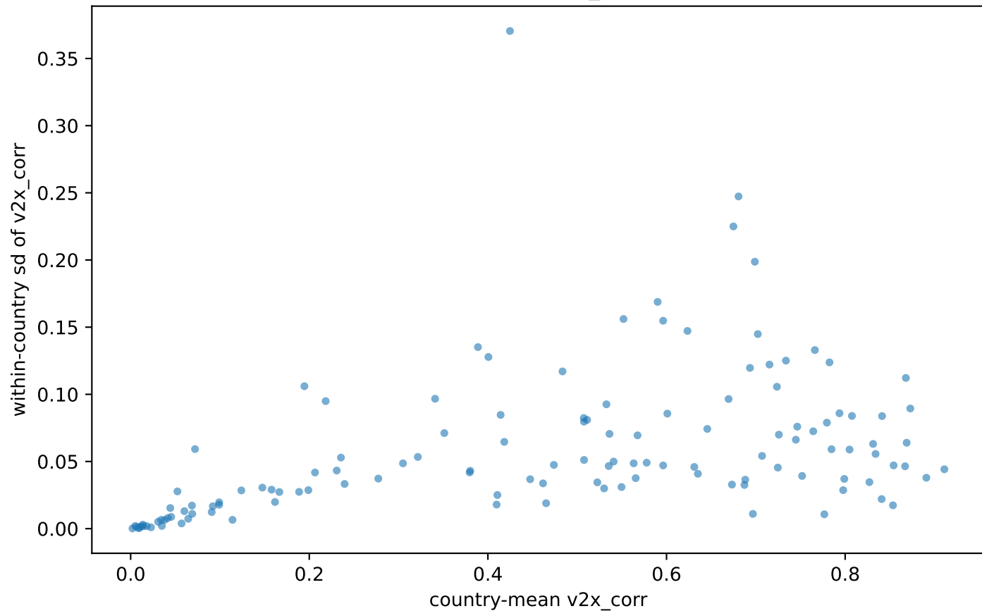
Between vs within variation: v2x_corr (n=128 countries)
