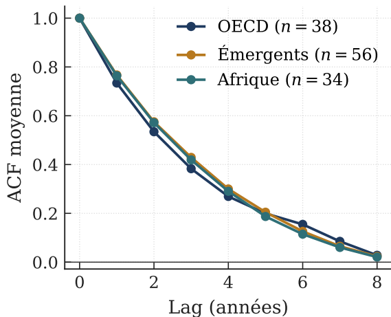
Corruption ( v2x_{\text{corr}} )
