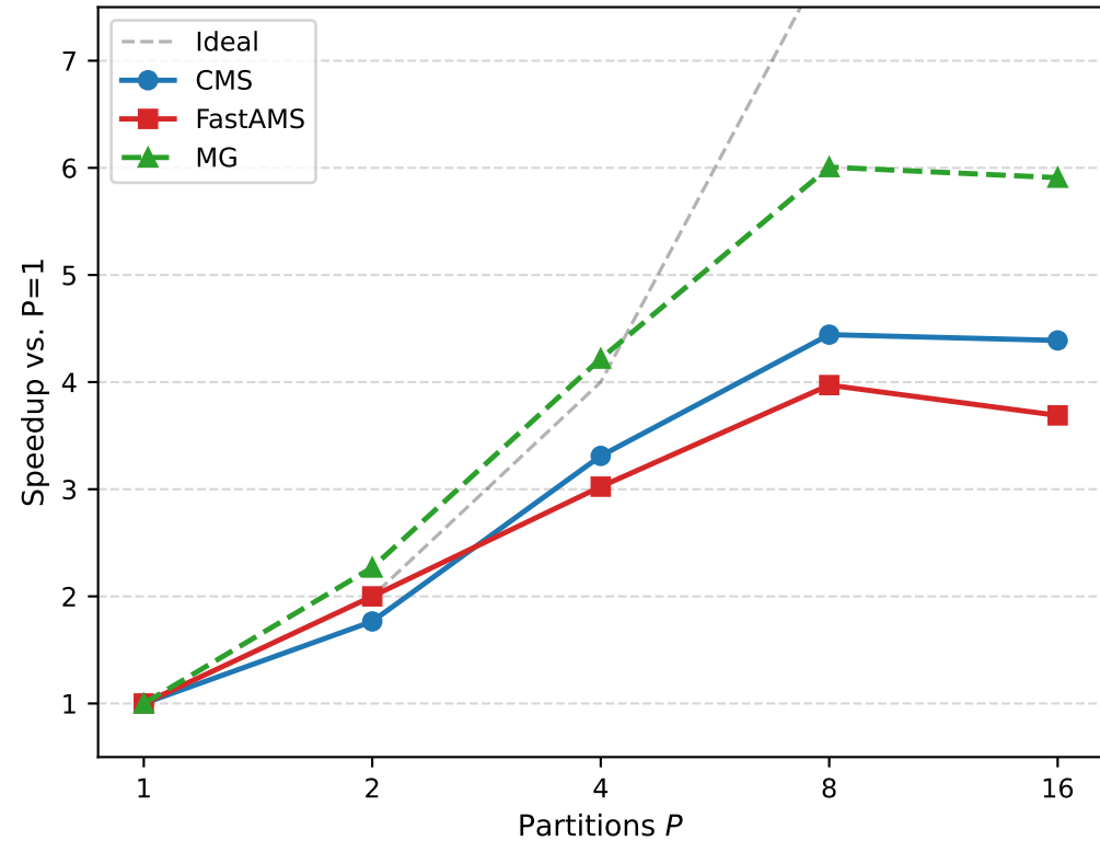
(a) Parallel speedup
