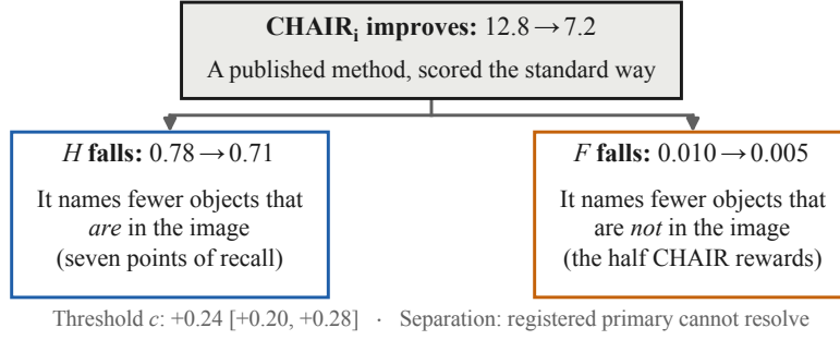
Figure 8: What the scalar score hides, on standard CHAIR: PAI’s CHAIR i improvement comes from naming fewer objects of both kinds. Numbers from Table 3.
