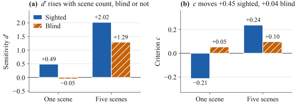
Figure 6: Signal-detection decomposition on LLaVA-1.5-7B. Sensitivity rises with scene count whether or not the image is present; the criterion moves mainly when it is.
