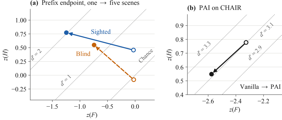
Figure 7: Operating points in z -coordinates. Dotted lines hold d' = z(H) - z(F) constant, so height above the chance diagonal is separation and movement parallel to it is a change of threshold. (a) The scene-count rise on LLaVA-1.5-7B, from one scene (open) to five (filled), moves away from the diagonal almost as far without the image as with it (post hoc for these conditions). (b) PAI on standard CHAIR moves almost parallel to the diagonal: on this probit scale the threshold changes and separation does not, although a logit separation measure does rise (Section 5).
