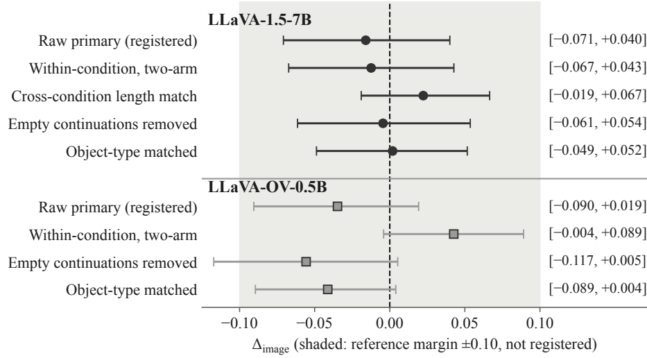
Figure 4: The image-attributable component on the two LLaVA-lineage architectures under every rule in Table 6, against the \pm 0.10 reference margin, which is a reporting choice rather than a registered bound. One interval, LLaVA-OV-0.5B’s with empty continuations removed, extends beyond the margin.
