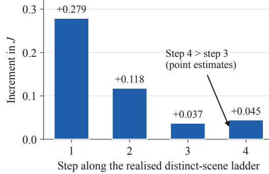
Figure 5: Increments in J along the realised distinct-scene ladder on LLaVA-1.5-7B. The first step carries 58% of the rise, so the curve is front-loaded; the fourth step’s point estimate slightly exceeds the third’s, so it shows no plateau within the grid. Distinct-type count and mentions-per-type track the manipulation with the same precision, so the ladder is graded in a quantity that co-varies with source-scene count rather than isolating it.
