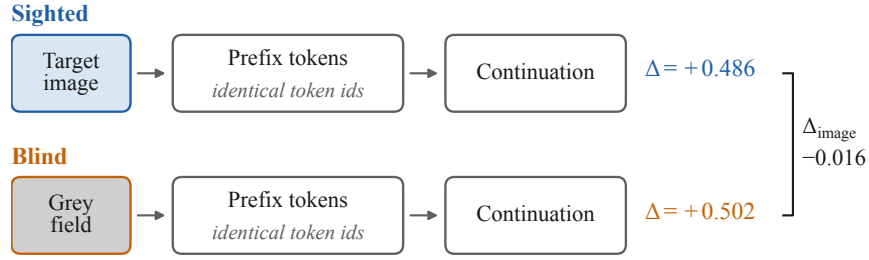
Figure 3: The design. The sighted and blind rows differ in the image alone; prefix token ids are bit-identical, so the difference between the two rises is attributable to replacing the image with a uniform grey field. On LLaVA-1.5-7B that difference is -0.016 .
