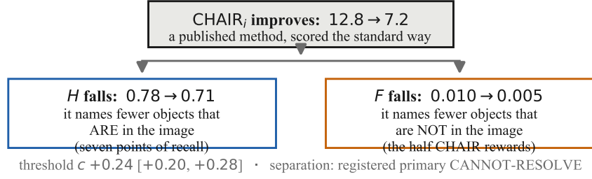
Figure 7: What the scalar score hides, on standard CHAIR: PAI’s CHAIR i improvement comes from naming fewer objects of both kinds. Numbers from Table 2.
