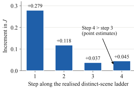
Figure 6: Increments in J along the realised distinct-scene ladder on LLaVA-1.5-7B. The first step carries 58% of the rise, so the curve is front-loaded; the fourth step’s point estimate slightly exceeds the third’s, so it shows no plateau within the grid. Distinct-type count and mentions-per-type track the manipulation with the same precision, so the ladder is graded in a quantity that co-varies with source-scene count rather than isolating it.
