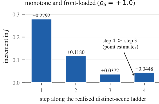
Figure 4: Increments in J along the realised distinct-scene ladder on the first architecture. The fourth step exceeds the third, so the curve is front-loaded rather than saturating. Distinct-type count and mentions-per-type track the manipulation with the same precision, so the ladder is graded in a quantity that co-varies with source-scene count rather than isolating it.
