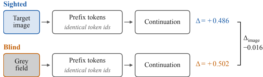
Figure 3: The design. The sighted and blind rows differ in the image alone; prefix token ids are bit-identical, so the difference between the two rises is attributable to replacing the image with a uniform grey field. On LLaVA-1.5-7B that difference is -0.016 .
