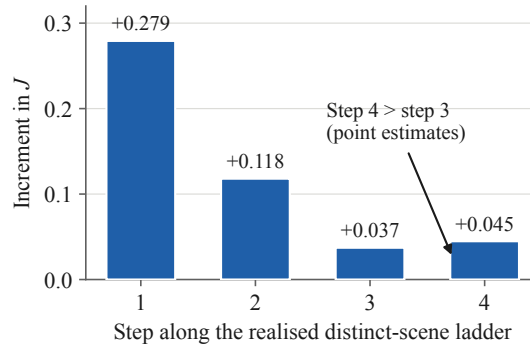
Figure 5: Increments in J along the realised distinct-scene ladder on LLaVA-1.5-7B. The first step carries 58% of the rise, so the curve is front-loaded; the fourth step’s point estimate slightly exceeds the third’s, so it shows no plateau within the grid. Distinct-type count and mentions-per-type track the manipulation with the same precision, so the ladder is graded in a quantity that co-varies with source-scene count rather than isolating it.
