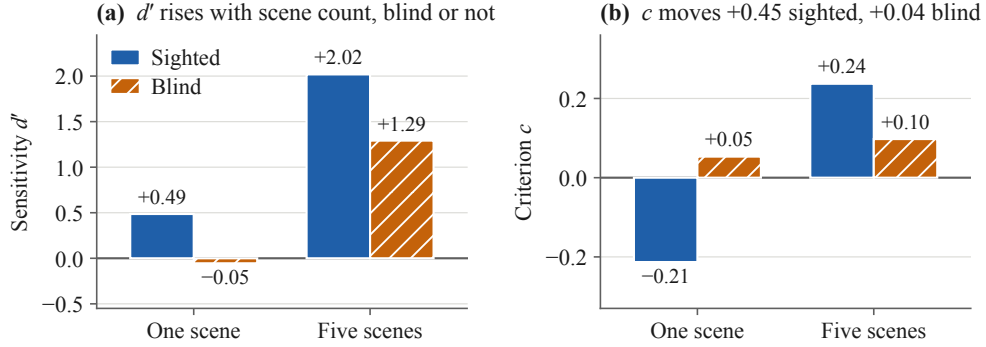
Figure 5: Signal-detection decomposition on LLaVA-1.5-7B. Sensitivity rises with scene count whether or not the image is present; the criterion moves mainly when it is.
