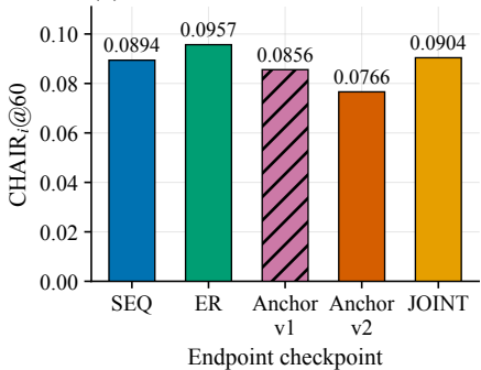
(b) Endpoint CHAIR i @60 (pilot only)
