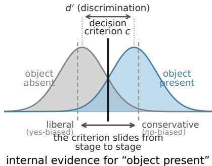
(a) Signal-detection schematic (not data)
