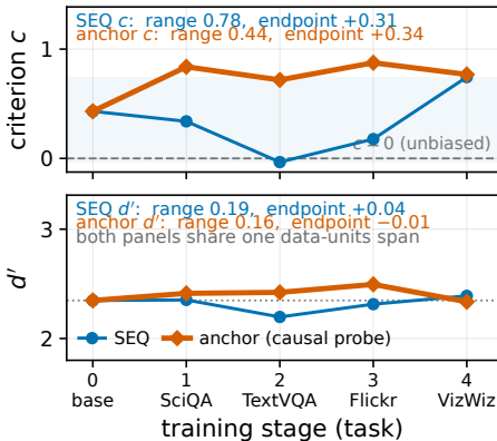
(b) PILOT: c range is 4.0\times the d' range
