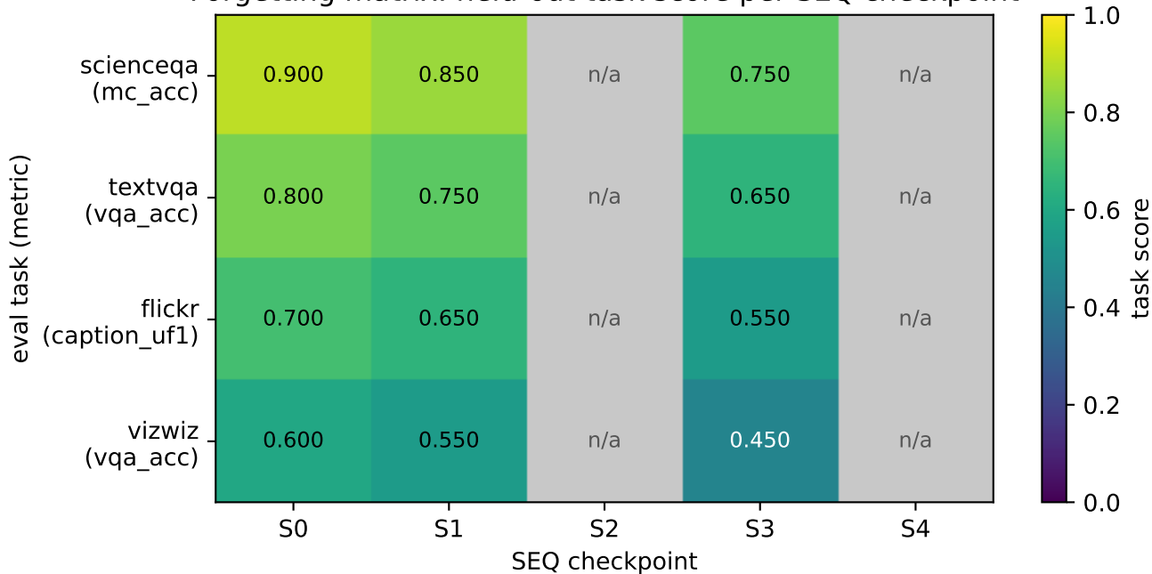
Forgetting matrix: held-out task score per SEQ checkpoint
