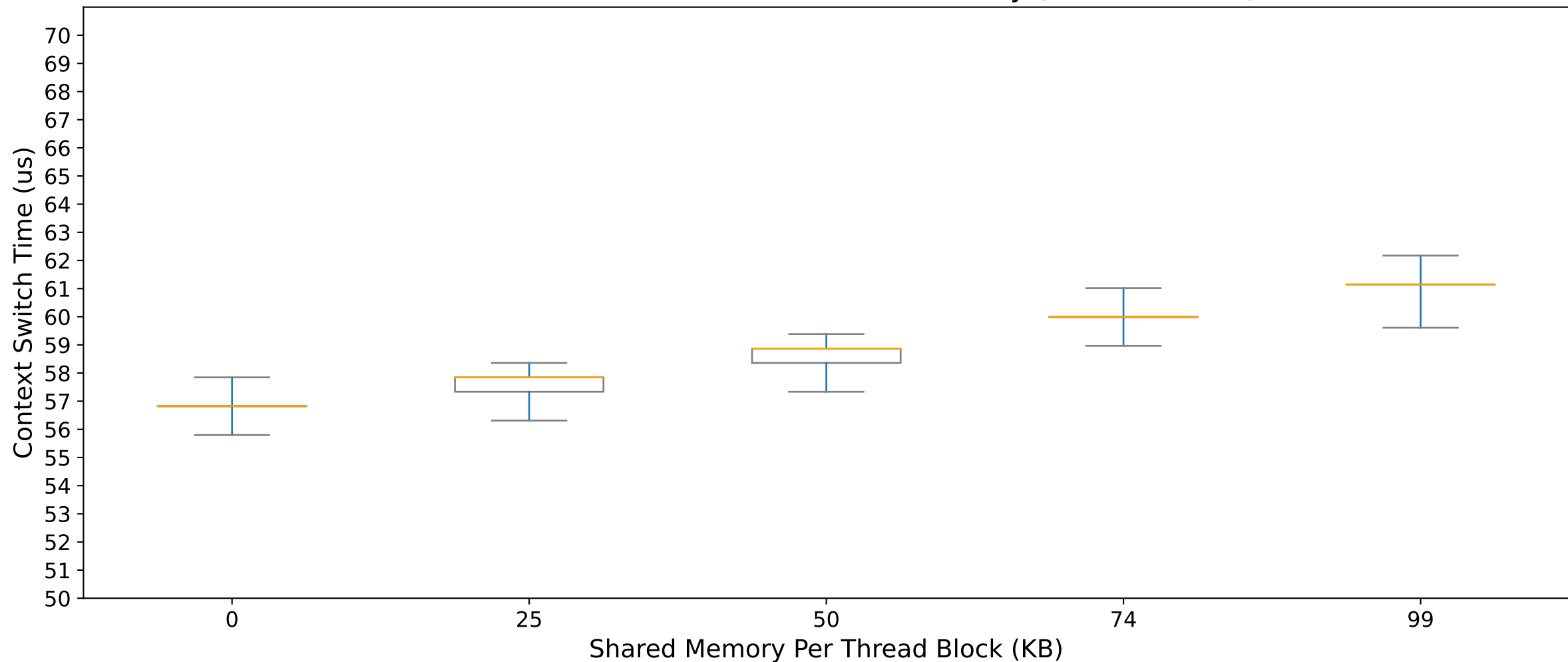
Context Switch Overhead of Shared Memory (RTX 6000 Ada)
