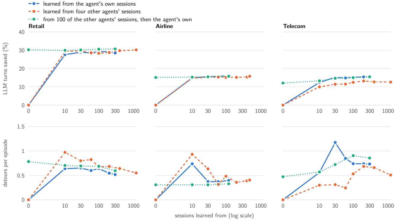
Figure 9. Turns saved (top) and detours per episode (bottom) against the sessions learned from, on a log scale: mean over three agents and three orders. The dotted line learns from 100 of the other agents' sessions, drawn at random, and the agent's first n .
