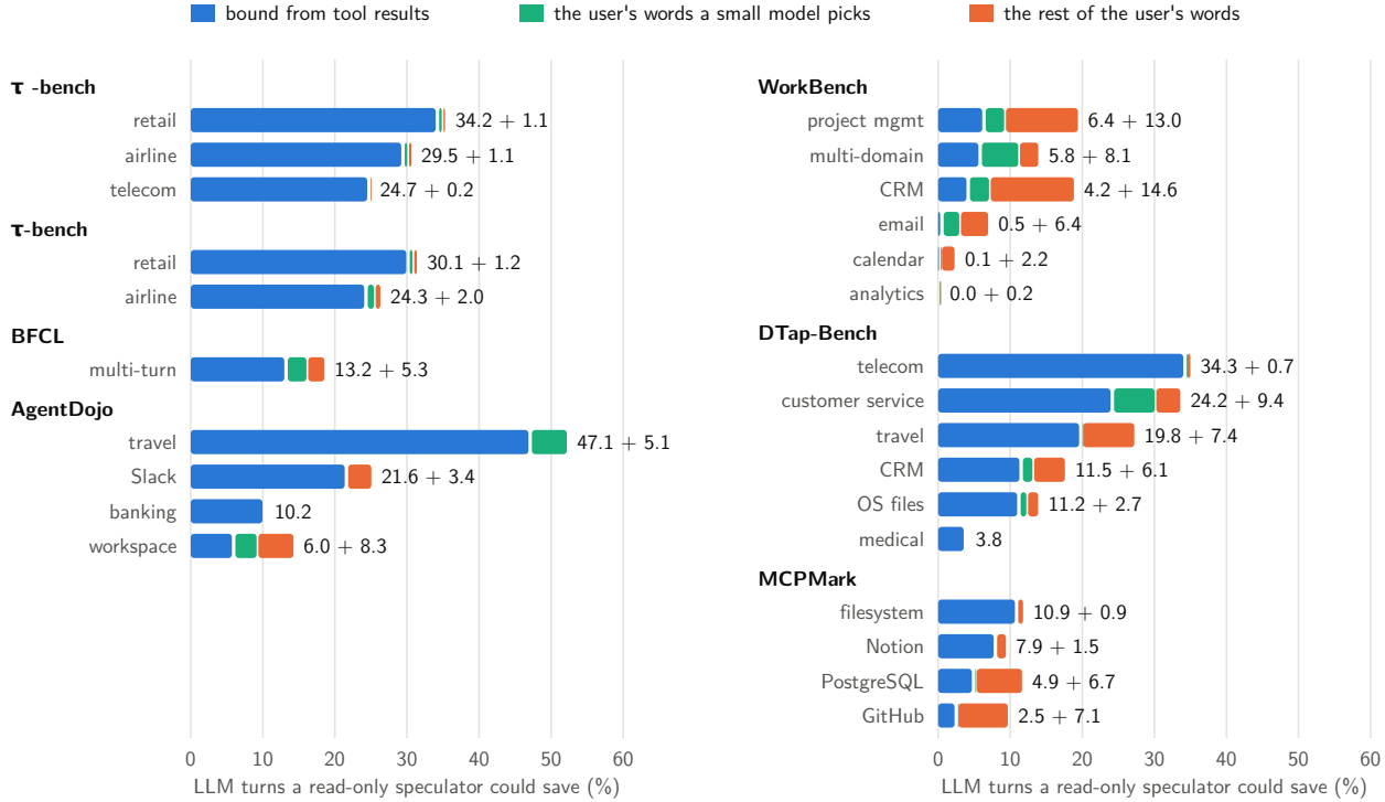
Figure 5. The read-only ceiling by benchmark and domain (test episodes of the replayed agents, §3), and on top what a speculator that also bound values from the user’s words could add: in green the values a small model, shown the user’s words and the call, picks among them (Appendix D), and in orange the rest. Where the agent walks records, results bind the arguments; where each request names what to read, only language does.
