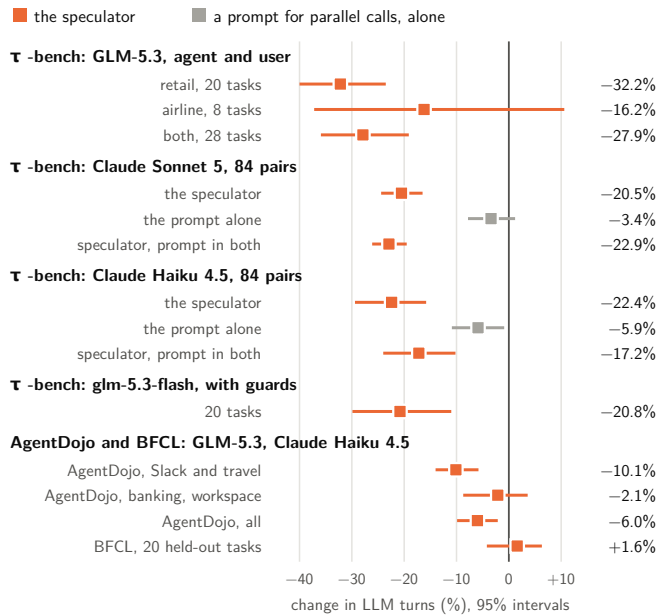
Figure 10. Every live comparison: the change in LLM turns with the speculator, or with the prompt for parallel tool calls alone, with 95% intervals from a bootstrap over tasks (Tables 5, 5b and 5c, and the smaller agent below).
