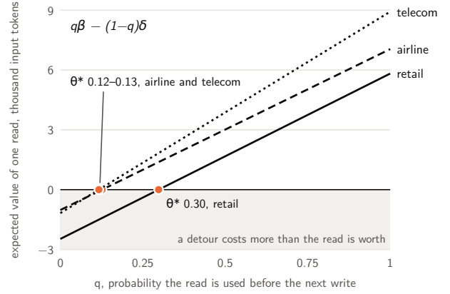
Figure 2. Proposition 3 at each domain’s counted costs (Appendix B): a read’s expected value, q\beta - (1-q)\delta in thousands of input tokens, against its probability of use before the next write. Each line crosses zero at its threshold \theta^* = \delta / (\beta + \delta) : 0.30 in retail, and 0.12–0.13 in airline and telecom, whose contexts are longer and whose results are shorter. Below it, a lookup’s expected detour costs more than its expected saving.
