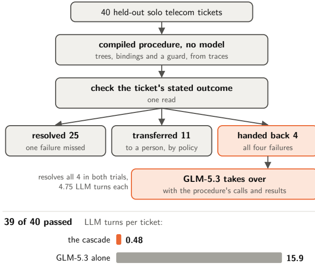
Figure 11. The cascade on solo telecom’s 40 held-out tasks (Table 6). The compiled procedure runs with no model, then checks the ticket’s stated outcome with a read: it judges 25 runs resolved (one of them a failure it misses), transfers 11 to a person as the policy directs, and hands back 4, all failures. GLM-5.3, given the procedure’s calls and results, resolved all four in both of two trials.
