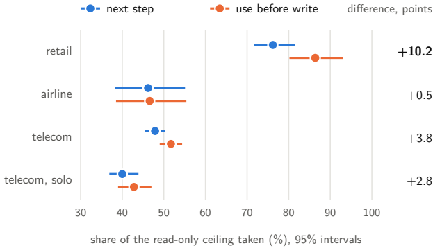
Figure 8. The share of the read-only ceiling each speculator takes in replay at \theta = 0.3 , nine agents’ test episodes (two in solo telecom), with 95% intervals from a bootstrap over tasks (Table 3). On the right, the use-before-write speculator’s lead, in points.
