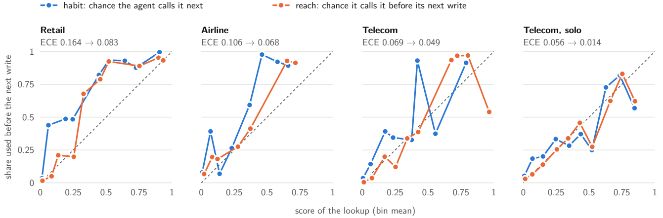
Figure 6. Reliability of the two scores (bins of at least 100 lookups). The next-step score sits above the diagonal: lookups it rates 0.4–0.6 are used nine times in ten.
