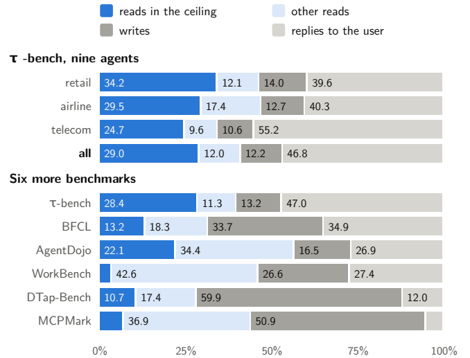
Figure 4. What decides each LLM turn, in \tau^2 -bench’s domains (Table 1) and six more benchmarks (Table 1b): reads in the ceiling, which a speculator binding from tool results could save (Proposition 2), other reads, writes, and replies to the user. Each bar is pooled over the test episodes of the replayed agents.
