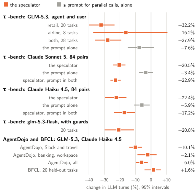
Figure 10. The live comparisons of the speculator of §2.4 and of the prompt for parallel tool calls: the change in LLM turns with the speculator, or with the prompt alone, with 95% intervals from a bootstrap over tasks (Tables 5, 5b and 5c, and the text below). GLM-5.3’s rows on \tau^2 -bench are against its recorded baseline.
