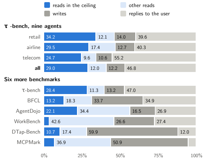
Figure 4. What decides each LLM turn, in \tau^2 -bench’s domains (Table 1) and six more benchmarks (Table 1b): reads in the ceiling, which a speculator binding from tool results could save at most (Proposition 2), other reads (the reads less the ceiling), writes, and replies to the user. Each bar is pooled over the test episodes of the replayed agents.
