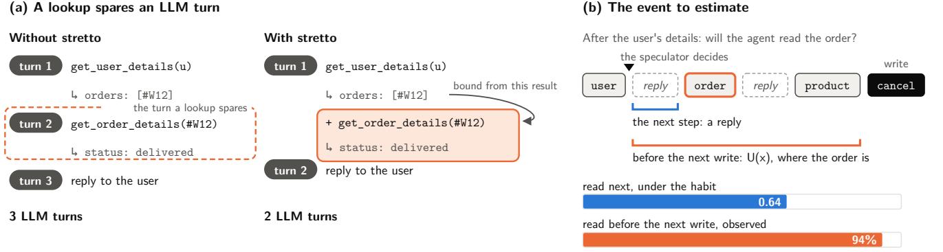
Figure 1. (a) A lookup spares an LLM turn. After the agent reads the user’s details, stretto reads the order they name, binding its id from that result, and appends what it returns to the same tool result: the agent has the order before it would ask for it. (b) The event to estimate. Here the agent’s next step is a reply, and it reads the order before its next write, the cancellation. After a user’s details, GLM-5 and Claude Sonnet 4.5 read an order next with probability 0.64 under the habit, but read it before their next write 94% of the time (§4.2). The calls are illustrative.
