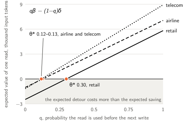
Figure 2. Proposition 3 at the counted costs of retail, airline and telecom (Appendix B): a read’s expected value, q\beta - (1 - q)\delta in thousands of input tokens, against its probability of use before the next write. Each line crosses zero at its threshold \theta^* = \delta / (\beta + \delta) : 0.30 in retail, and 0.12–0.13 in airline and telecom, whose contexts are longer and whose results are shorter. Below it, a lookup’s expected detour costs more than its expected saving.
