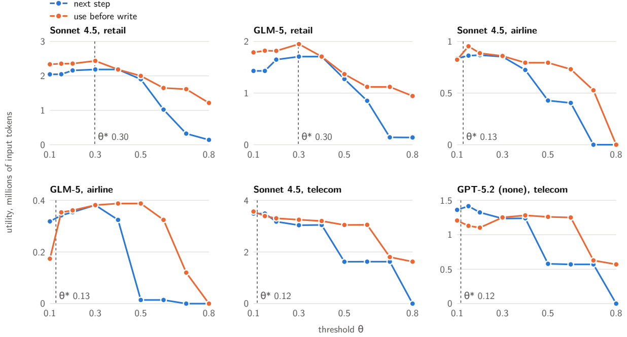
Figure 4. Utility against the threshold, in millions of the agent’s input tokens at its domain’s counted costs, on the test episodes of GLM-5 and Claude Sonnet 4.5 (retail, airline, telecom) and GPT-5.2 without reasoning (telecom), for speculators learned from the 2025 runs; the dashed line is the domain’s \theta^* . Every cell is in the round’s published rows.
