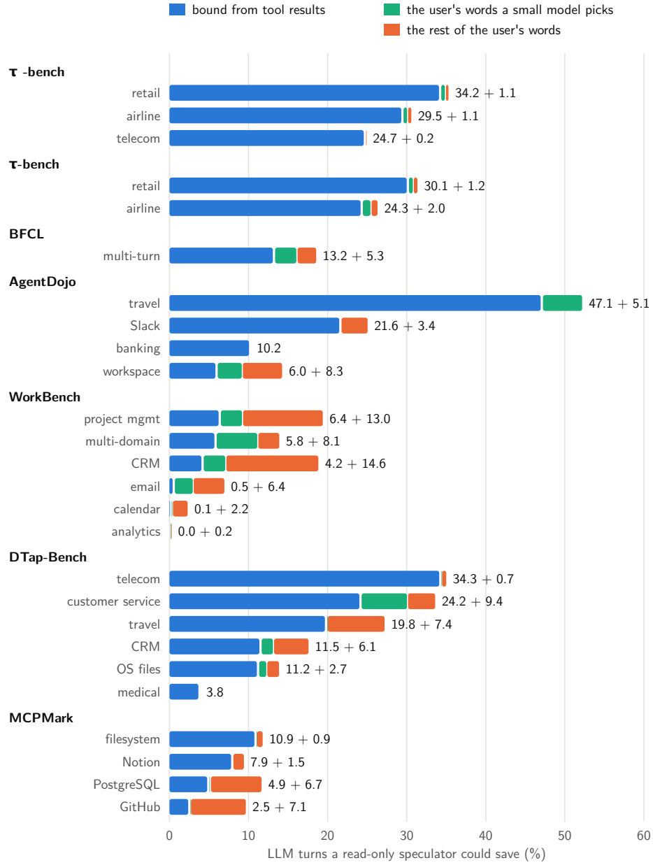
Figure 2. The read-only ceiling by benchmark and domain (test episodes of the replayed agents, §3), and on top what a speculator that also bound values from the user’s words could add: in green the values a small model, shown the user’s words and the call, picks among them (Appendix D), and in orange the rest. Where the agent walks records, results bind the arguments; where each request names what to read, only language does.
