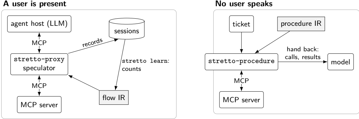
Figure 1. The two regimes in stretto. Left: the proxy forwards every message, records sessions, and after each of the agent’s calls makes the lookups the flow decides on, inside the same tool result. Right: a compiled procedure runs with no model and hands a ticket to one only when its check of the stated outcome fails.
