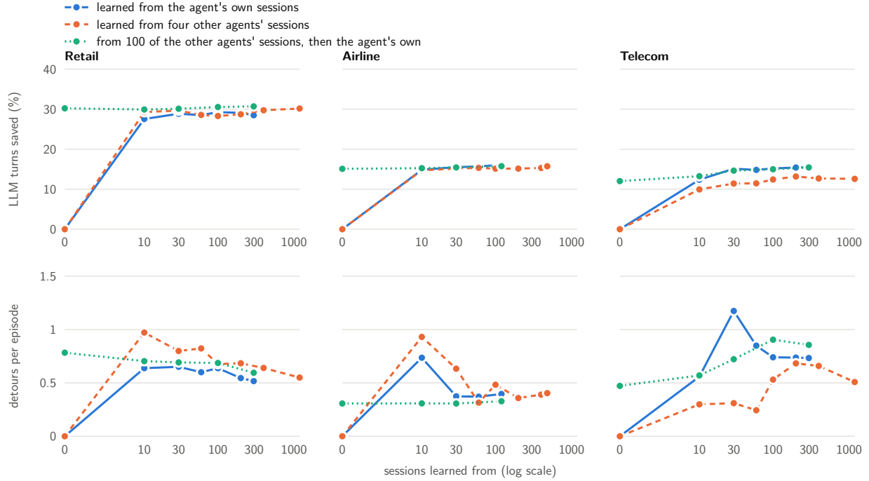
Figure 5. Turns saved (top) and detours per episode (bottom) against the sessions learned from, on a log scale: mean over three agents and three orders. The dotted line learns from 100 of the other agents’ sessions, drawn at random, and the agent’s first n .
