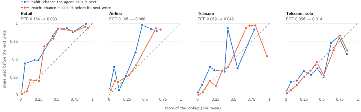
Figure 3. Reliability of the two scores (bins of at least 100 lookups). The next-step score sits above the diagonal: lookups it rates 0.4–0.6 are used nine times in ten.
