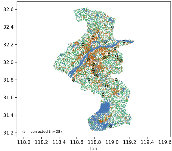
Nanjing — LOCO-corrected ( \tau=0.85 , lowest 10% margin)
