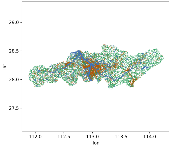
Changsha — WorldCover (raw)
