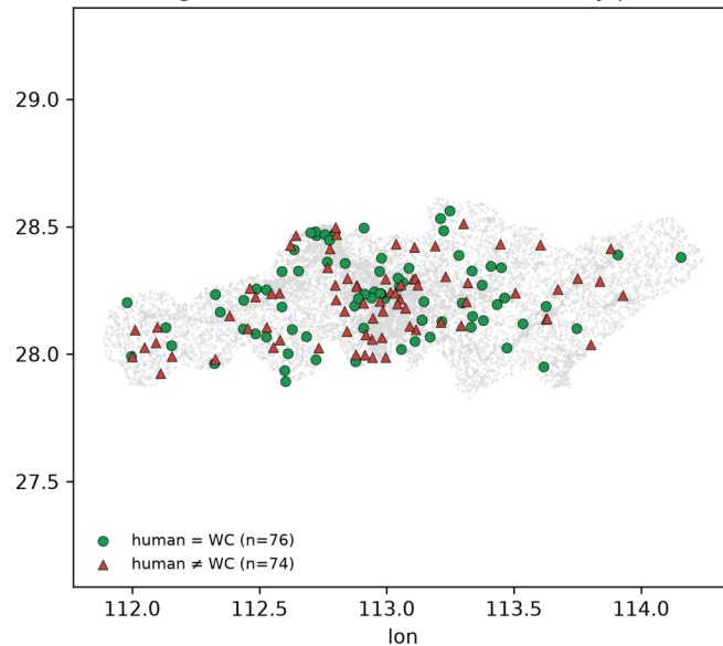
Changsha — 150 hand-labelled boundary points
