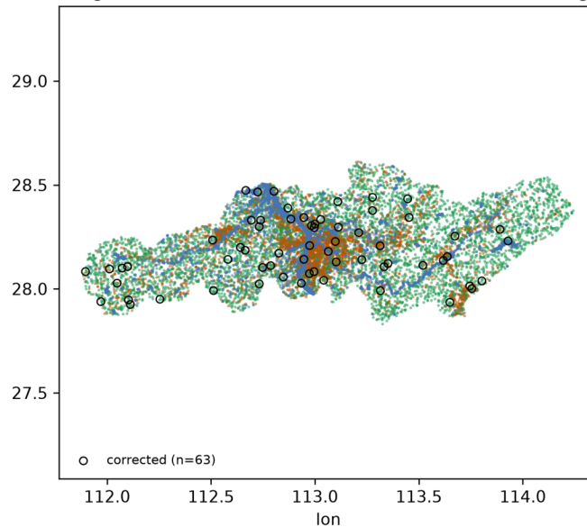
Changsha — LOCO-corrected ( \tau=0.85 , lowest 10% margin)
