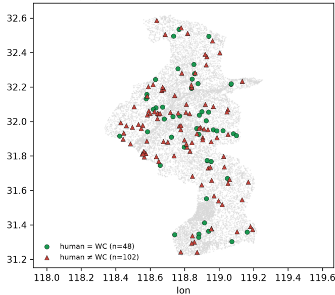
Nanjing — 150 hand-labelled boundary points
