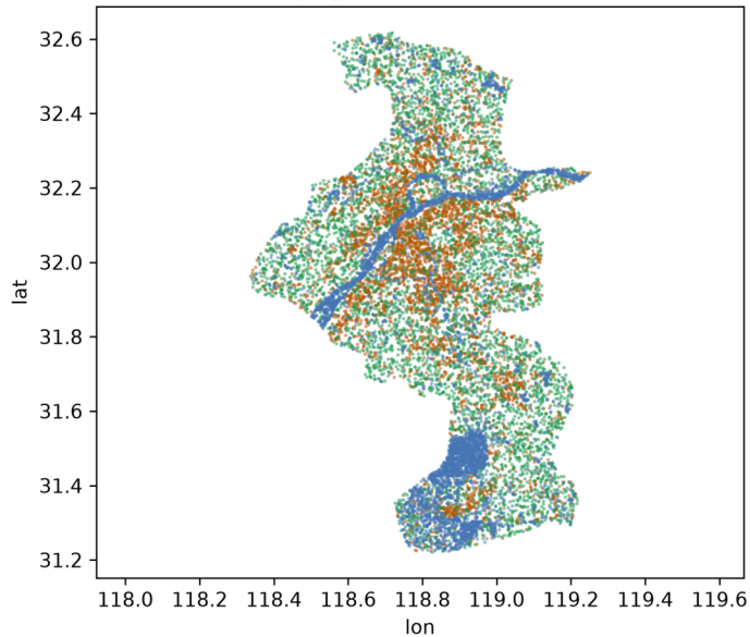
Nanjing — WorldCover (raw)
