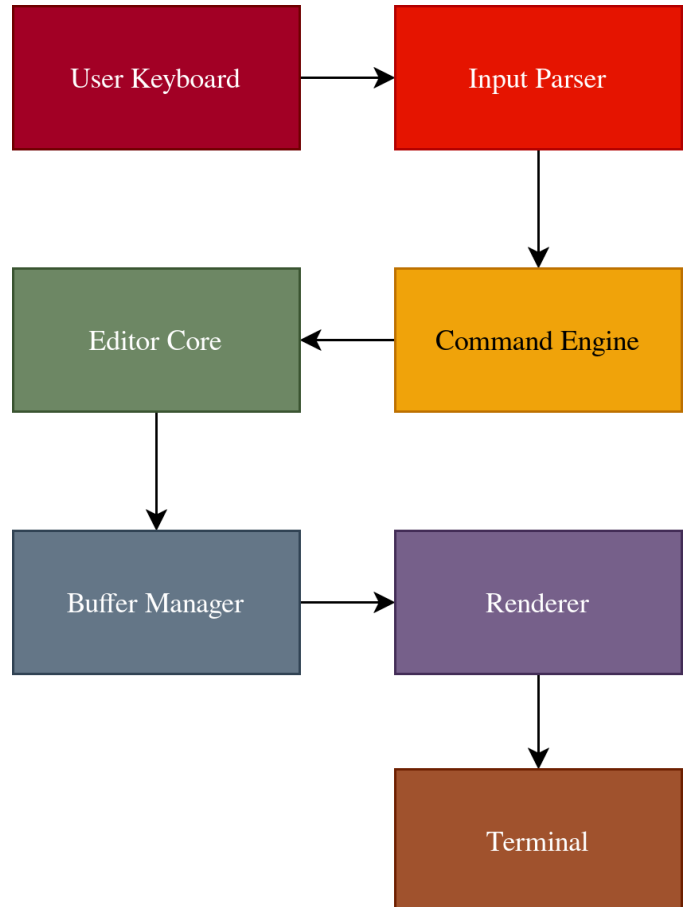
Fig. 1. High-level system architecture of VIP.
