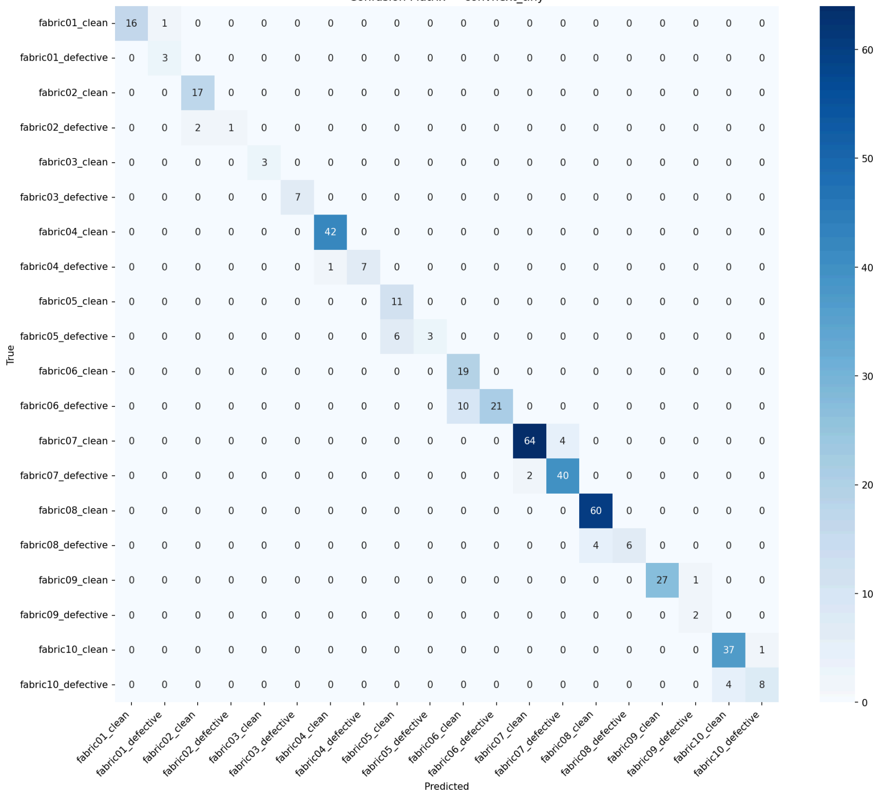
Confusion Matrix — convnext_tiny
