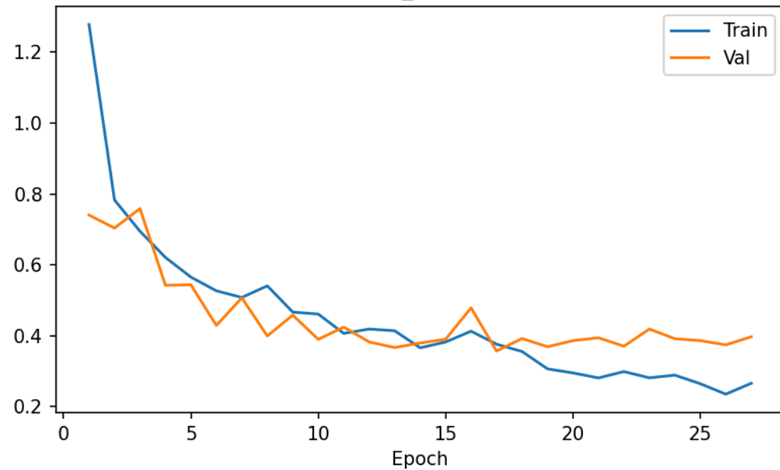
convnext_tiny — Loss
