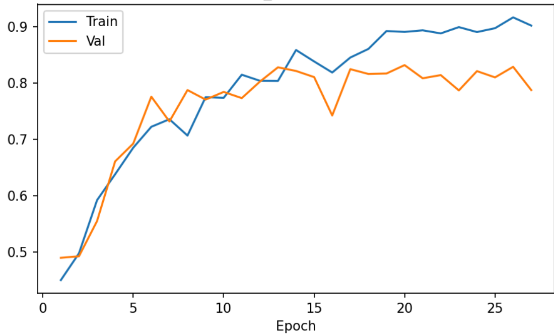
convnext_tiny — Macro-F1
