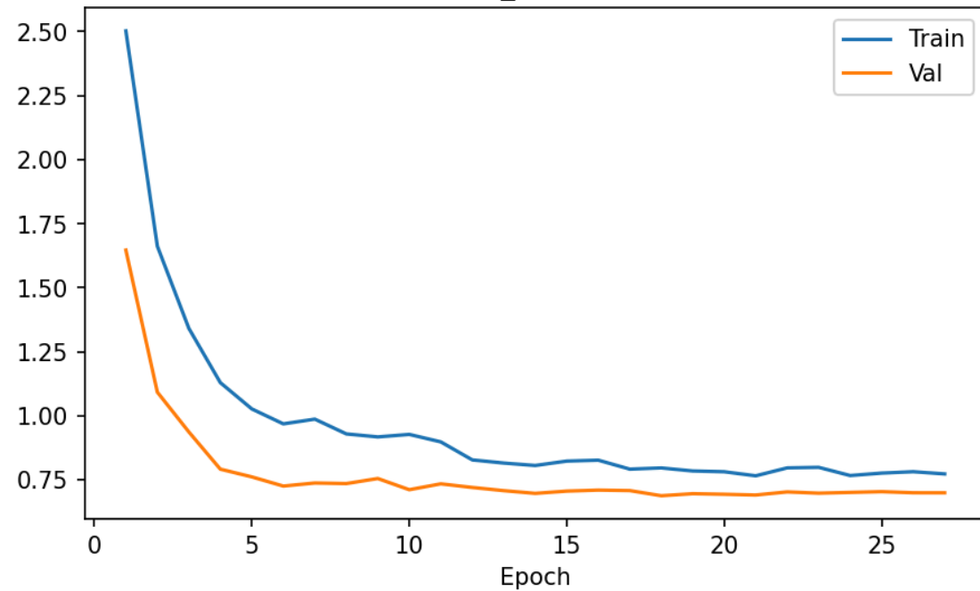
custom_cnn — Loss
