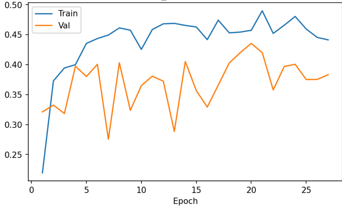
custom_cnn — Macro-F1
