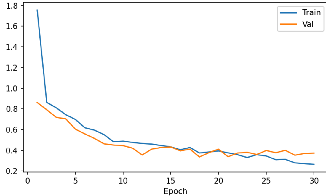
efficientnet_v2_s — Loss
