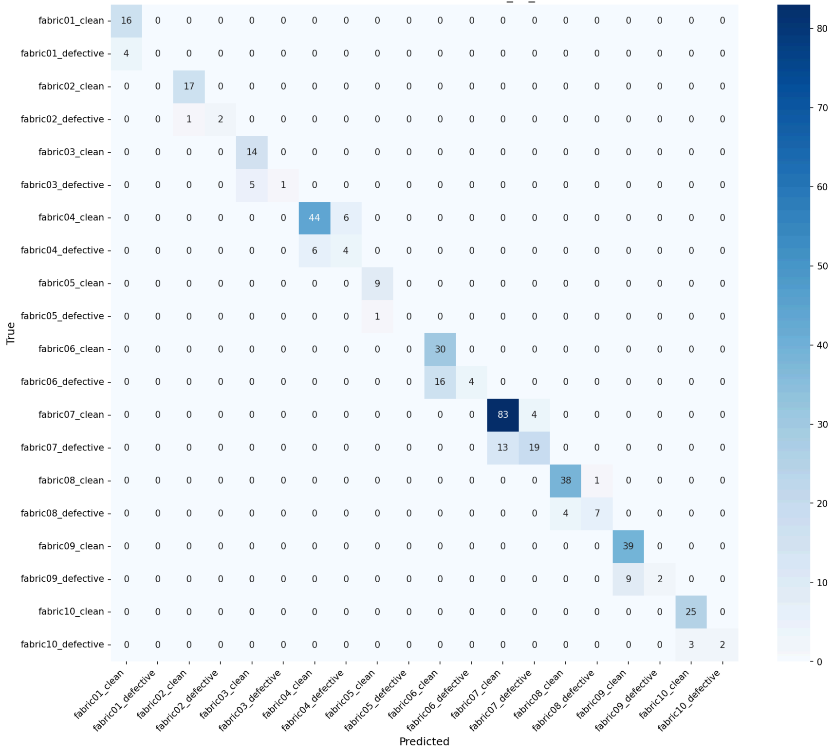
Confusion Matrix — efficientnet_v2_s
