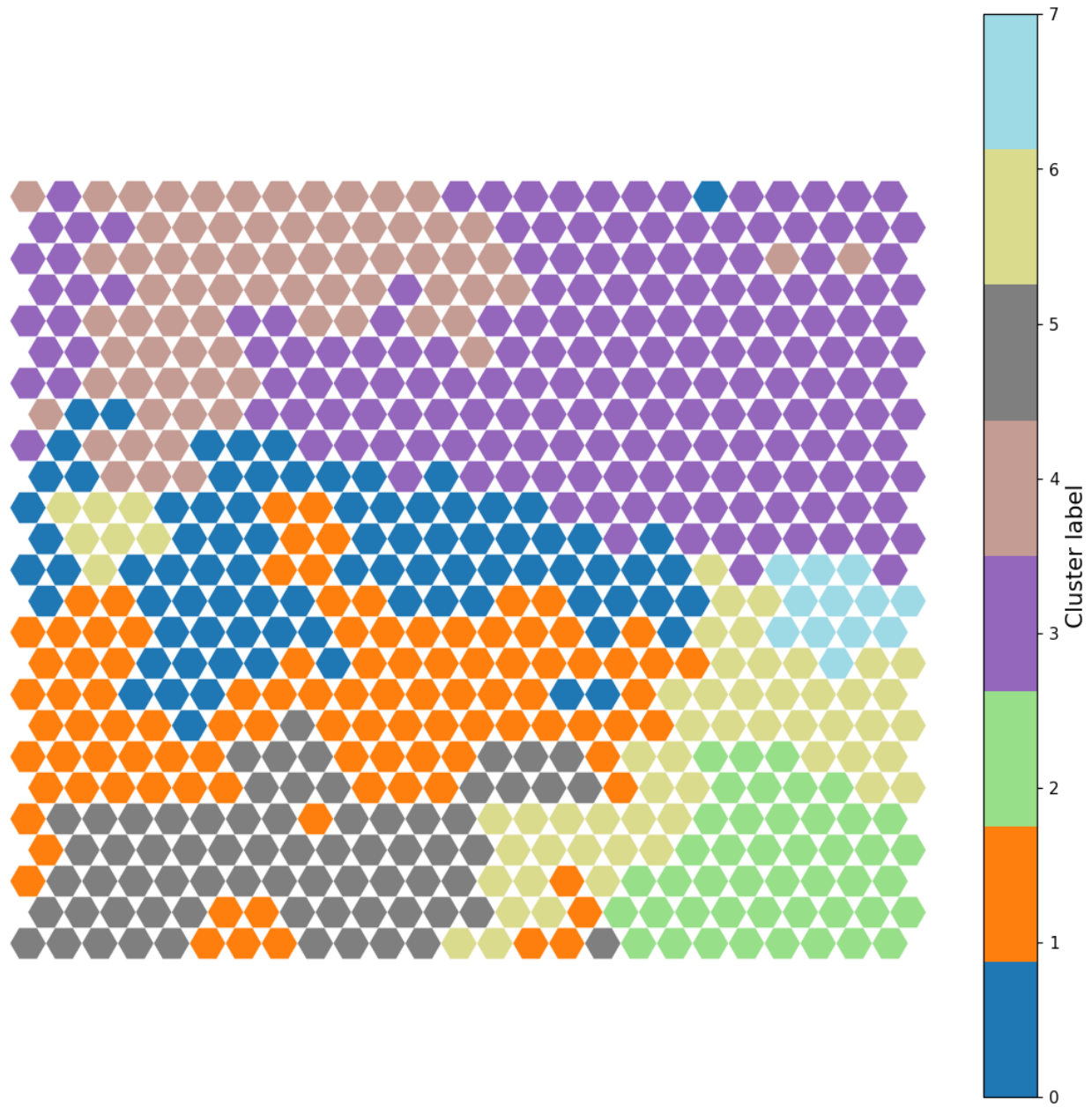
KMEANS Clusters 25x25 — 8 clusters
