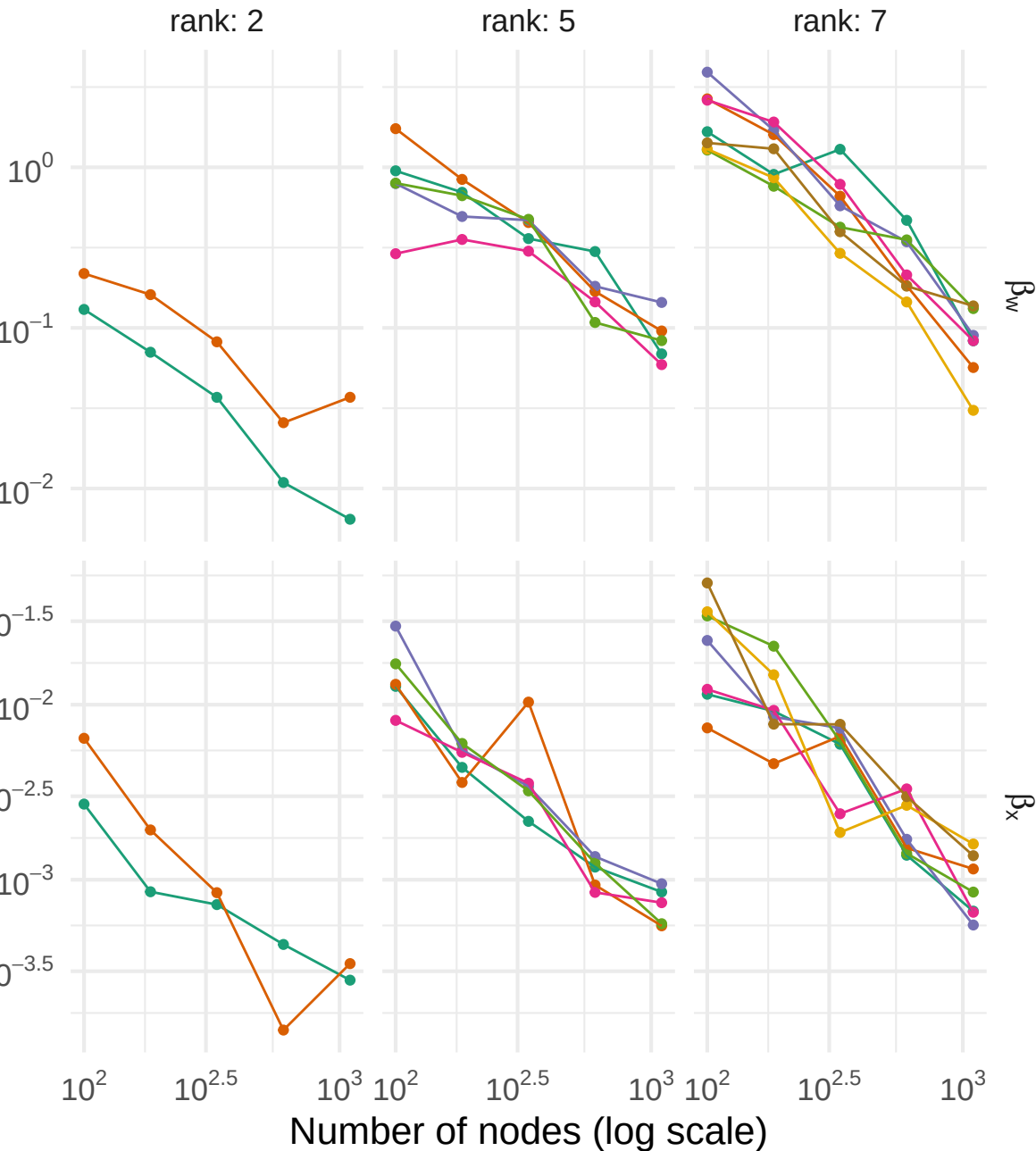
Mean squared error (log scale, after procrustes alignment)
