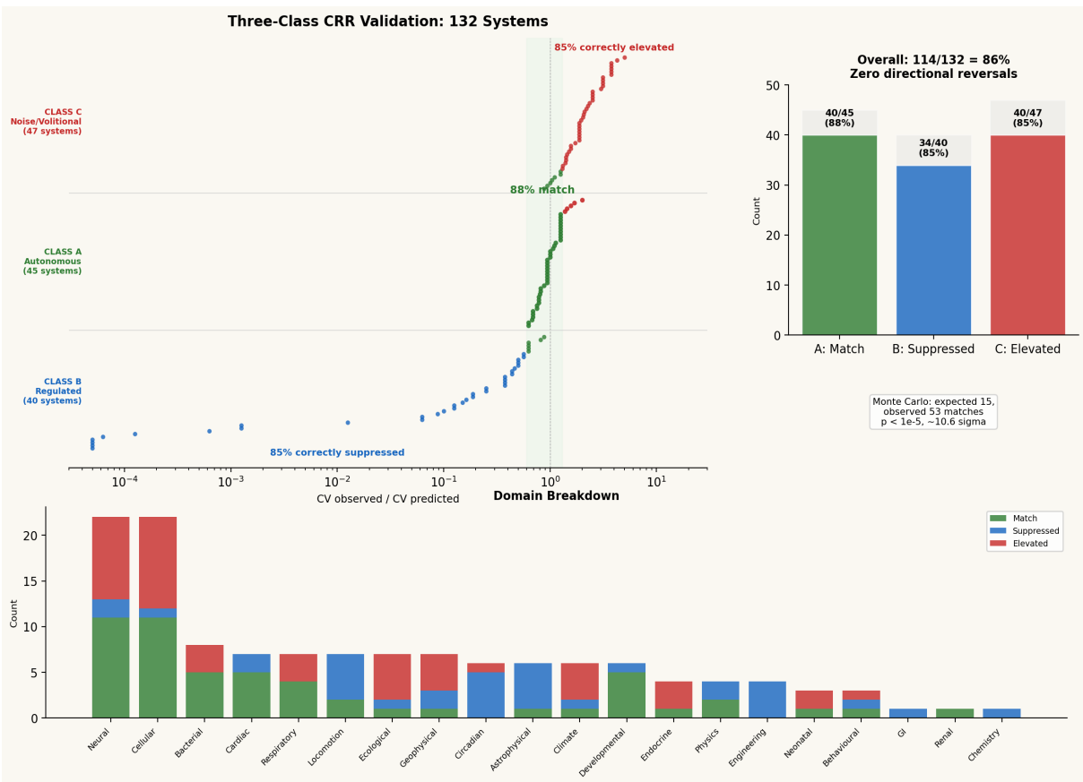
Figure 1. Three-class CRR validation across 132 systems. Top left: ratio strip plot (CV observed / CV predicted) grouped by class. Green band marks the match zone [0.6\times, 1.3\times] . Top right: three-class prediction accuracy with Monte Carlo significance. Bottom: domain breakdown showing match (green), suppressed (blue), and elevated (red) systems per domain.
