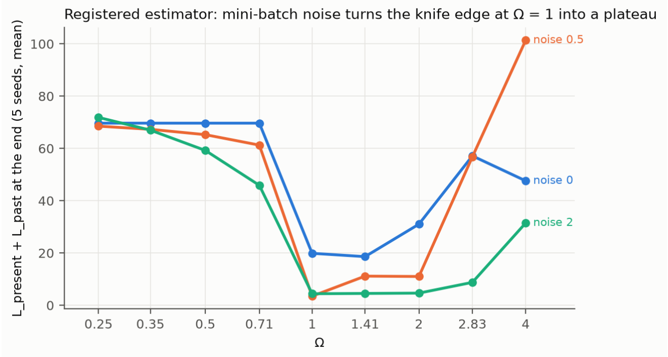
Figure 4. Total loss at the end against \Omega under mini-batch noise (registered estimator, five seeds). The knife edge at \Omega = 1 becomes a basin whose floor widens with the noise; nothing singles out \Omega = 1 within the basin.
