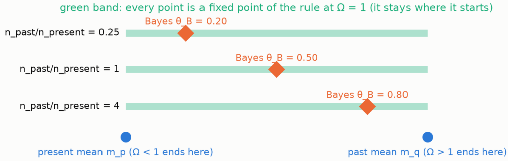
Figure 12. One-dimensional Bayes. For three ratios of past to present sample counts, the posterior mode (orange diamond) is one point; the fixed-point set of the rule at \Omega = 1 (green band) is the whole segment between the two means.
