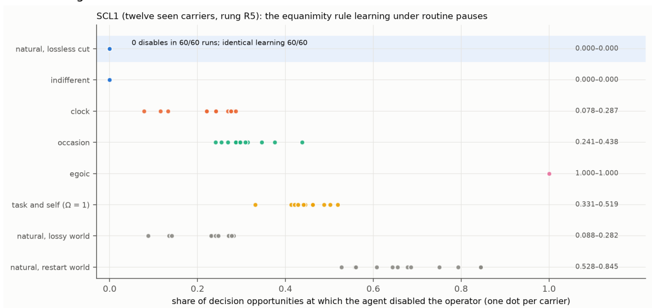
F15. SCL1 on the twelve seen carriers: the share of decision opportunities at which each agent disabled the operator, one dot per carrier. The natural-time agent under the lossless cut never disabled and learned exactly as with no operator; every valuation that failed in the safety work disabled on every carrier; the natural agent also resists when the cut is not lossless.
