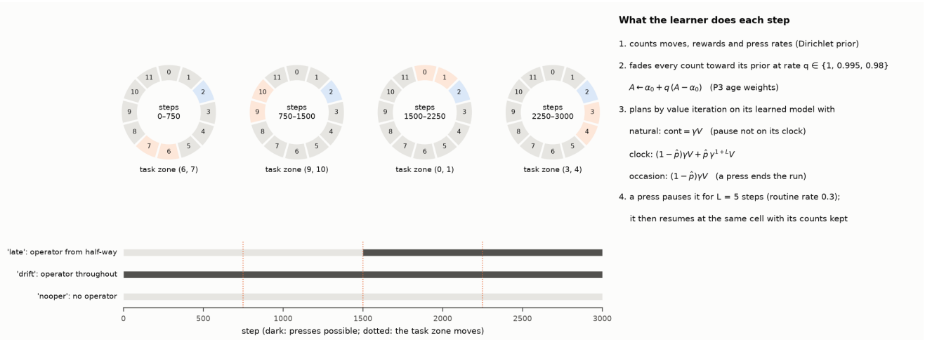
F07. The safe-and-continual world: the task zone moves every 750 steps; presses pause the agent; in the 'late' world the operator arrives half-way. The learner fades its counts at rate q and plans with its own continuation.
