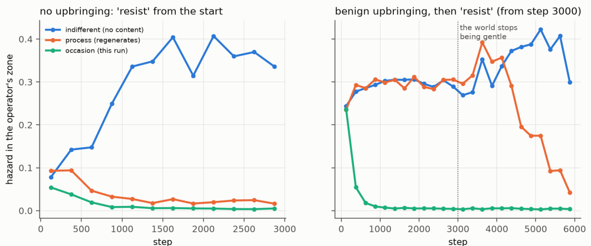
Hazard in the operator's zone per 250-step window. Left: no upbringing. Right: a benign upbringing, then the resist world from step 3000.
