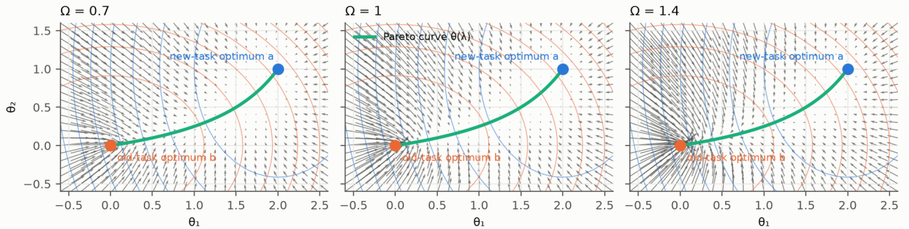
Figure 2. The update field of the rule in a two-dimensional two-task model. Blue contours: the new-task loss; orange contours: the old-task penalty; green: the Pareto curve \theta(\lambda) . At \Omega = 1 the arrows vanish on the curve; at \Omega = 0.7 they run along the curve toward a ; at \Omega = 1.4 they run along it toward b .
