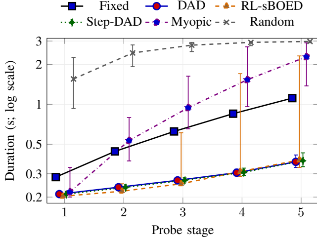
Fig. 2. IEEE 14-bus pulse durations at T = 5 : medians and interquartile ranges for all six methods. Fixed and learned methods: 4608 histories over three seeds; Myopic and Random: 1536 each. Horizontal offsets separate methods. Bars show pooled variation, not confidence intervals; ordering is imposed.
