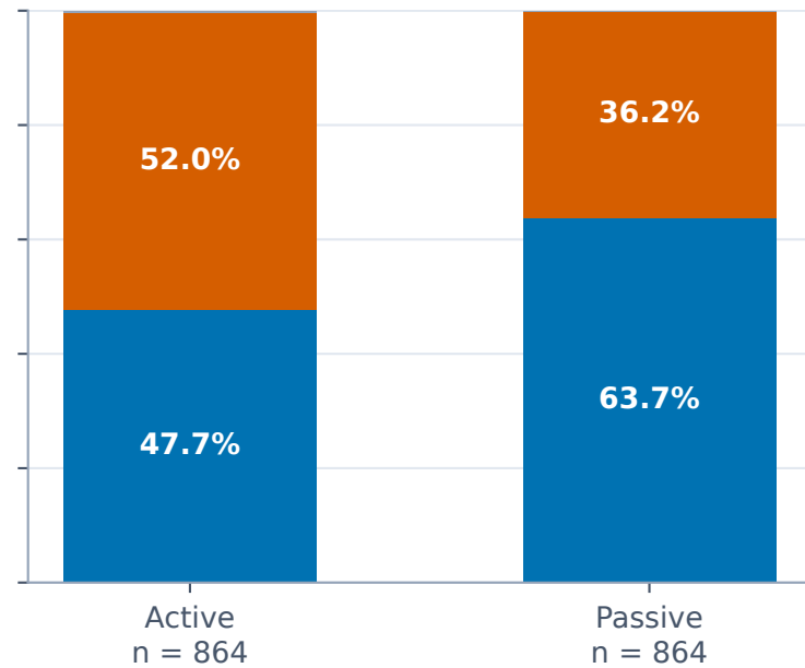
Generalization test
