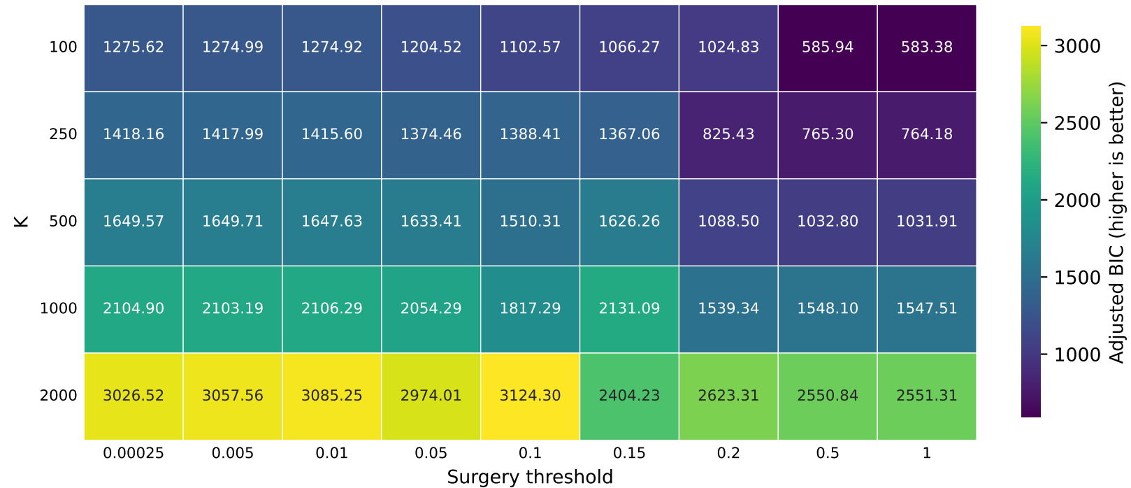
Adjusted BIC
