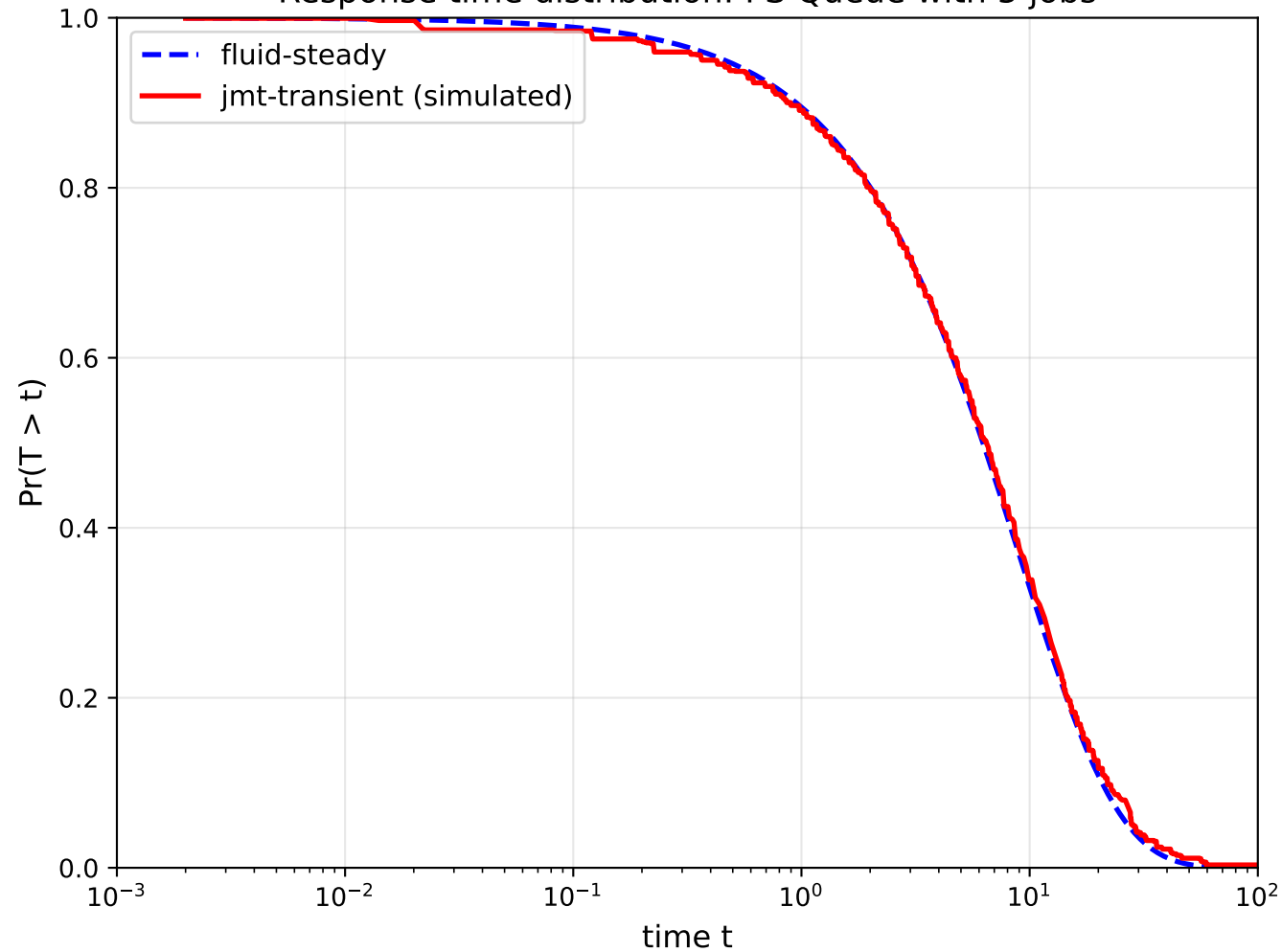
Response time distribution: PS Queue with 5 jobs
