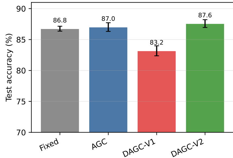
FashionMNIST + CNN SGD, lr=0.4
