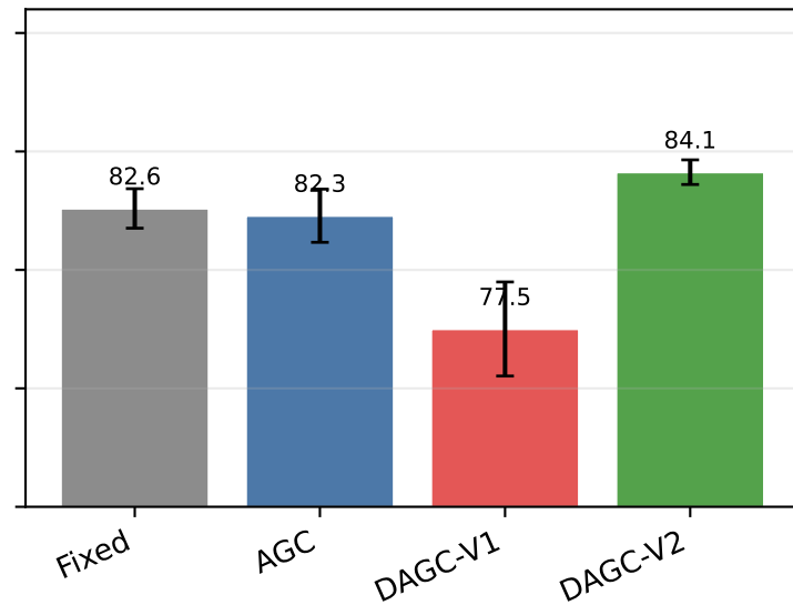
FashionMNIST + MLP SGD, lr=0.8
