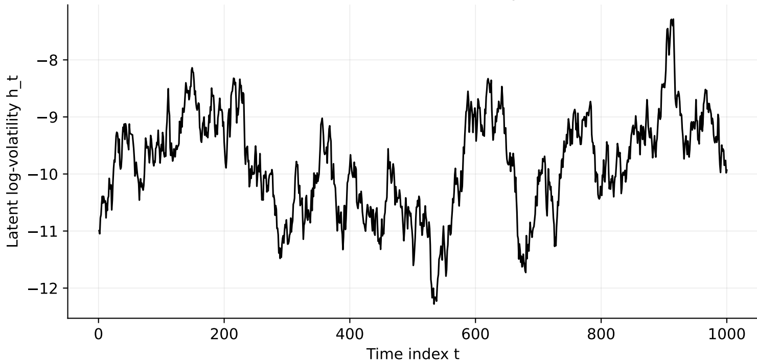
Simulated Latent Volatility
