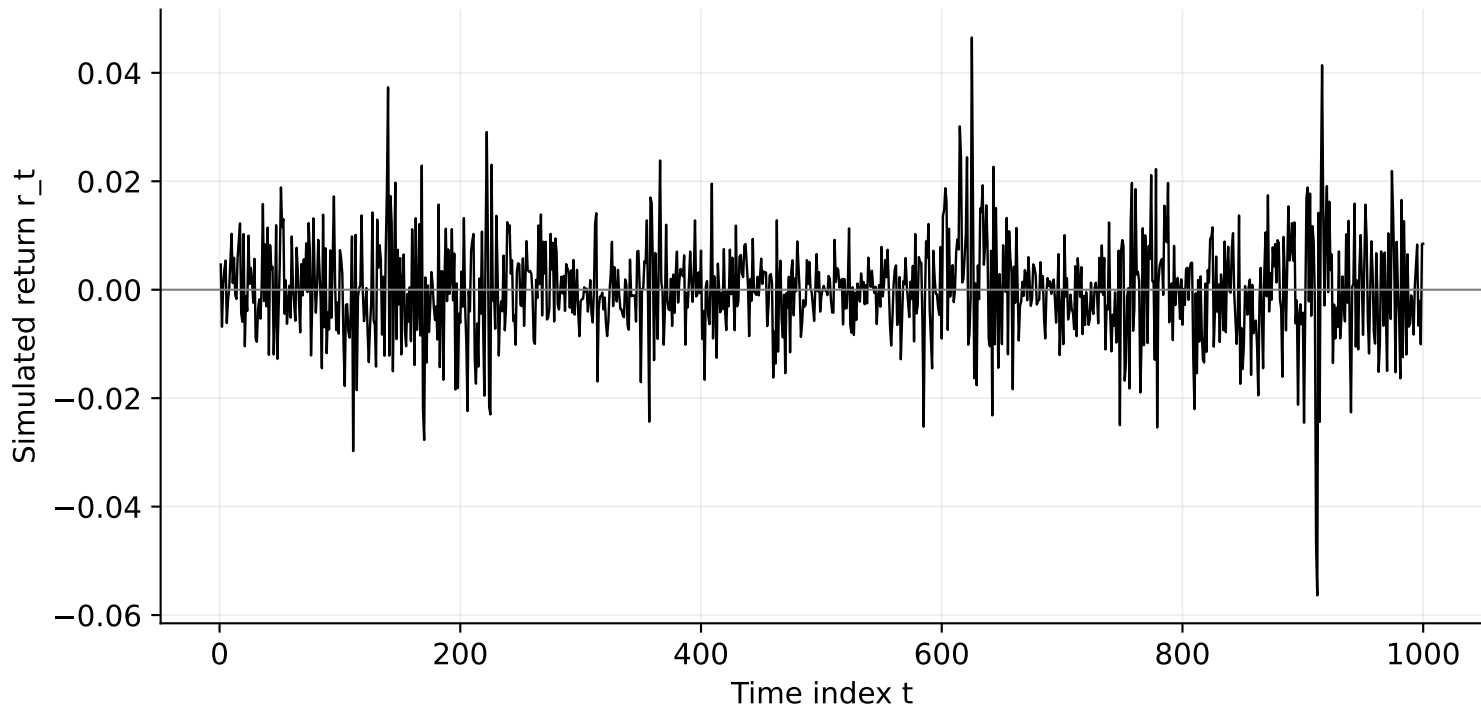
Simulated Returns from the SV Model
