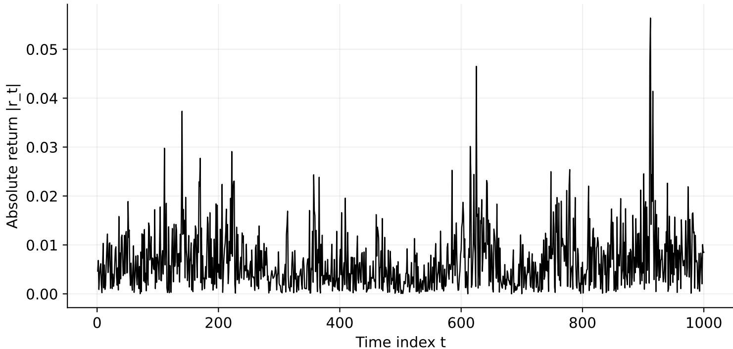
Absolute Returns and Volatility Clustering
