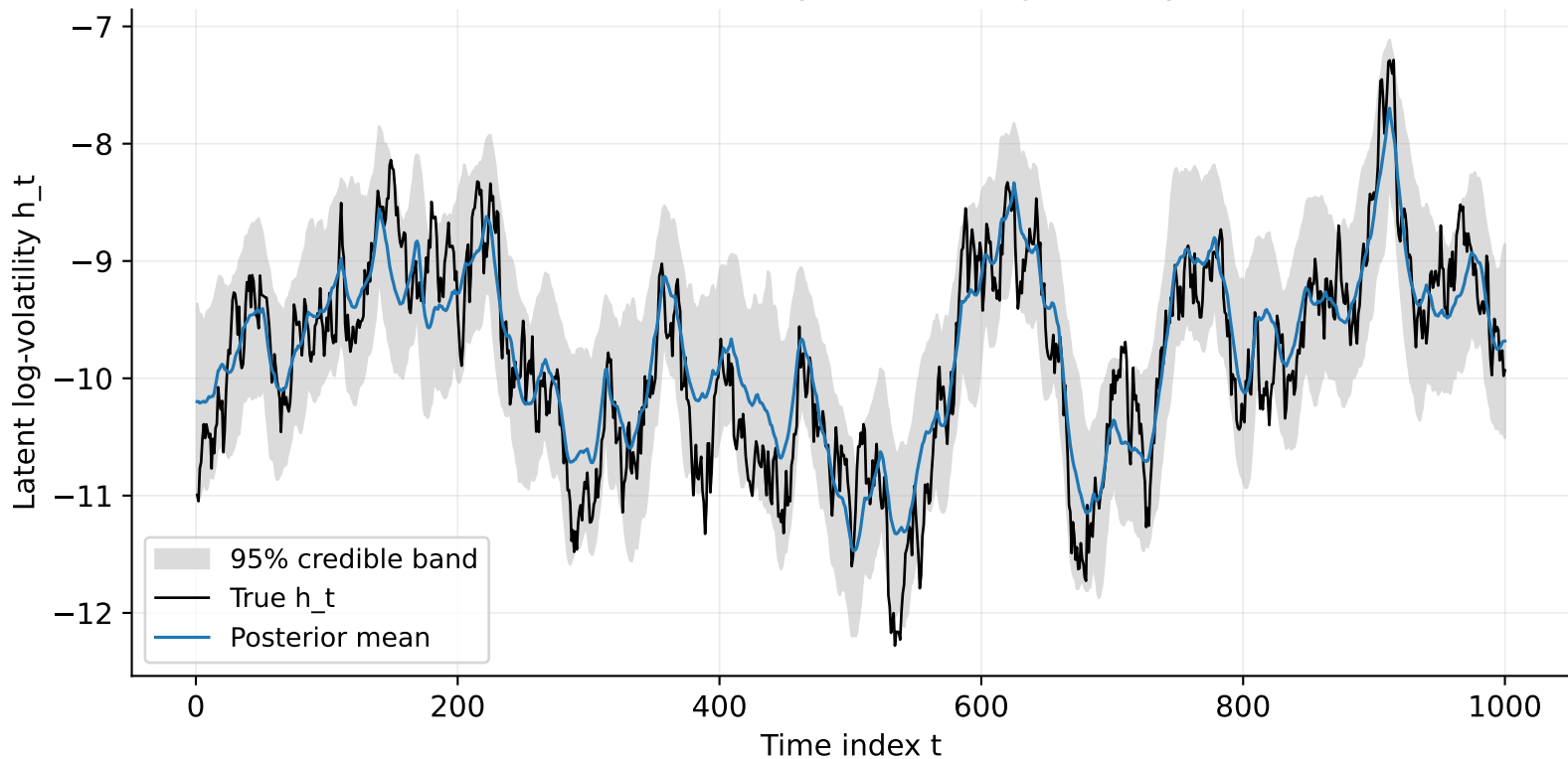
Posterior Recovery of Latent Log-Volatility
