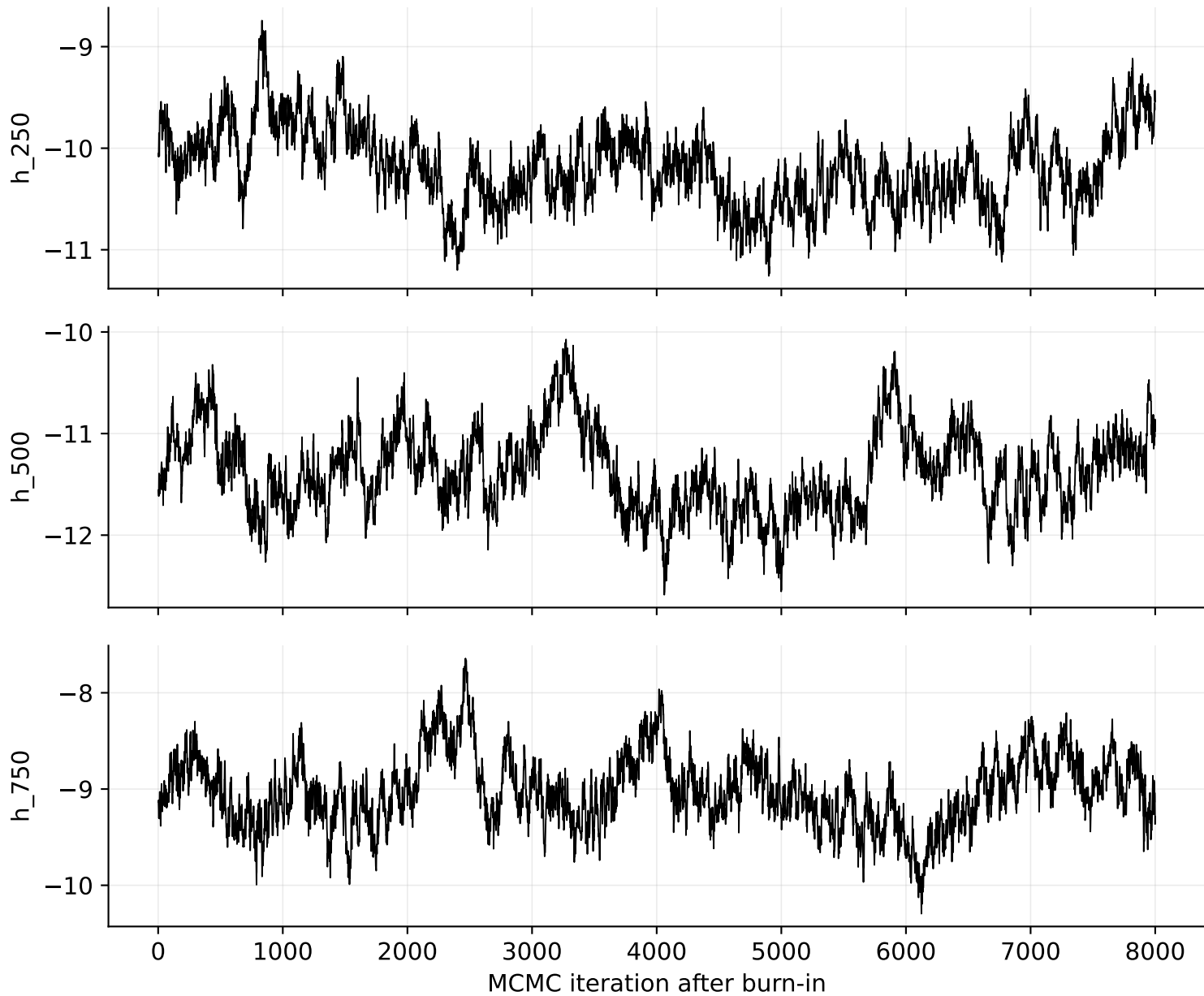
Trace Plots for Selected Latent States
