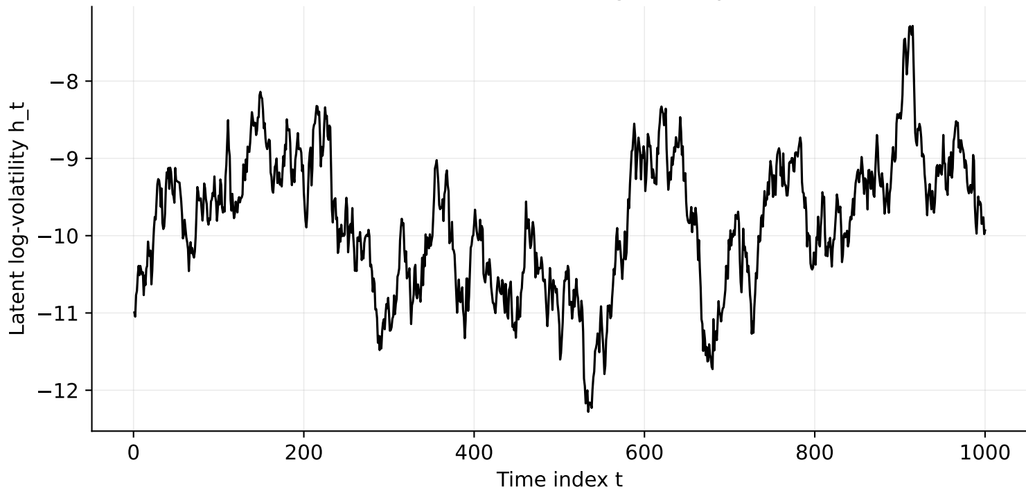
Simulated Latent Log-Volatility
