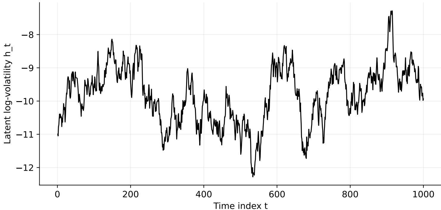
Simulated Latent Volatility
