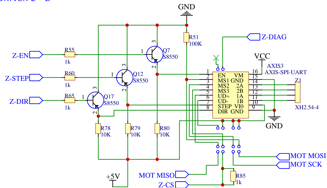
DRIVER 2 - Z
