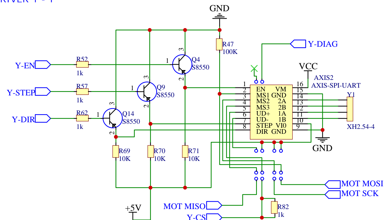
DRIVER 1 - Y
