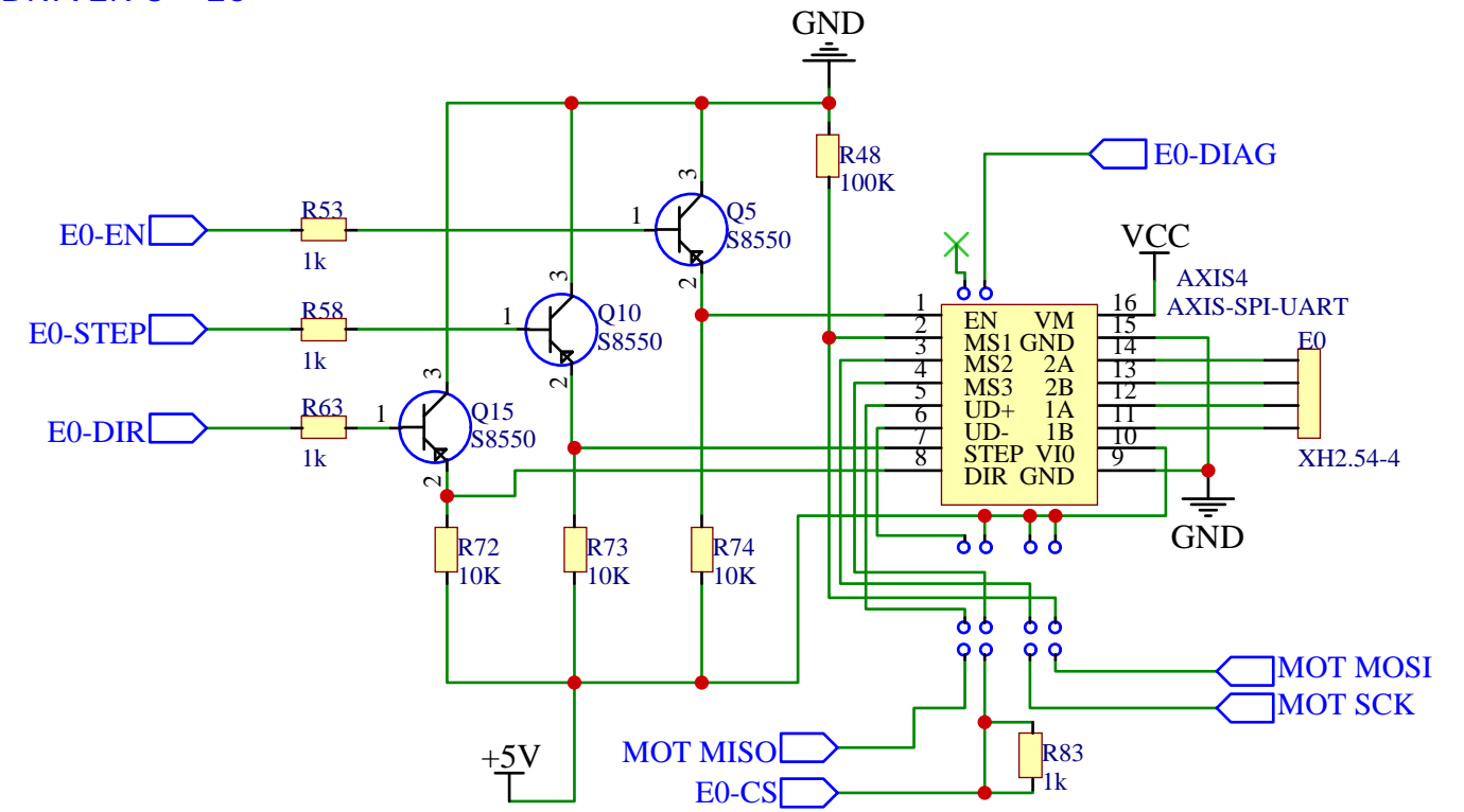
DRIVER 3 - E0
