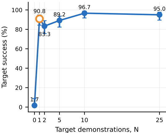
(a) One demo reaches the high-success regime
