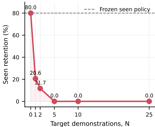
(b) The same adaptation forgets seen skills
