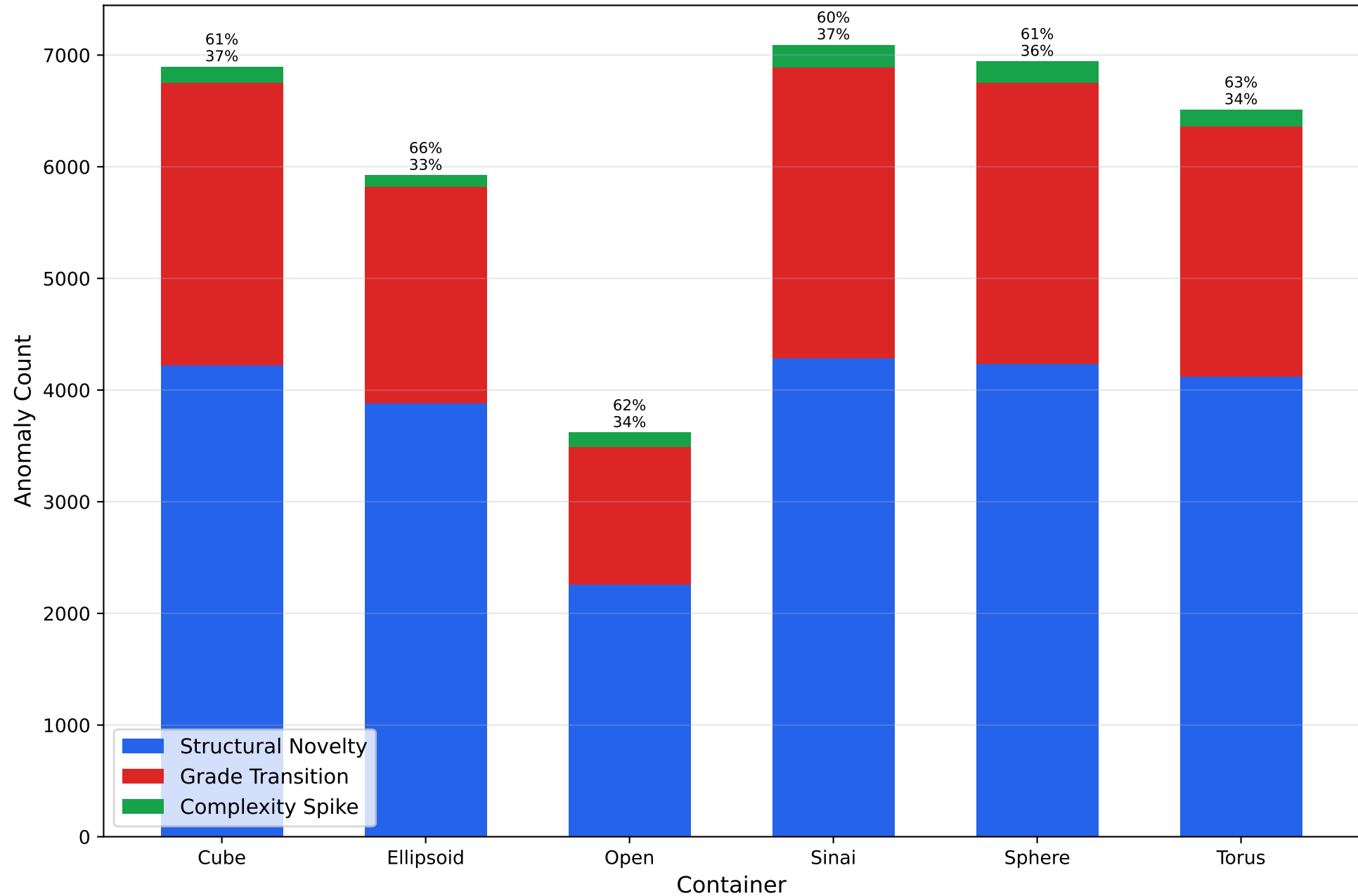
Anomaly Type Breakdown by Container
