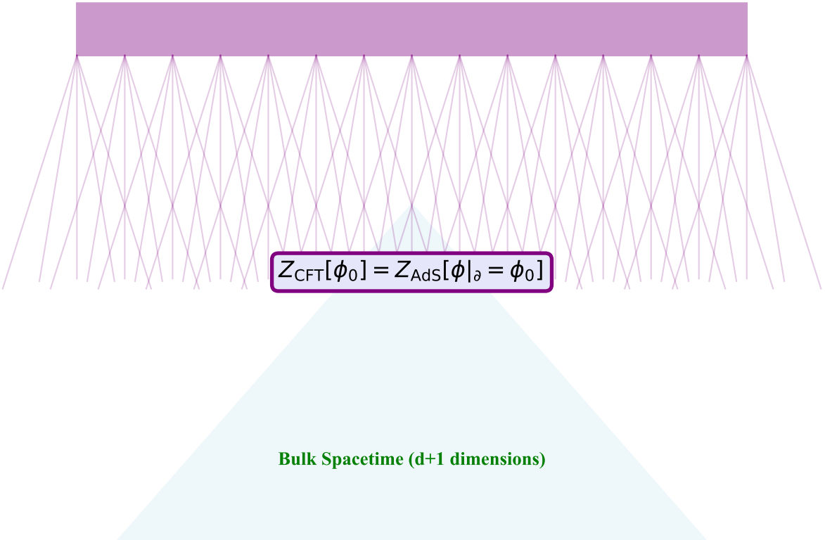
Holographic Projection: Boundary → Bulk
