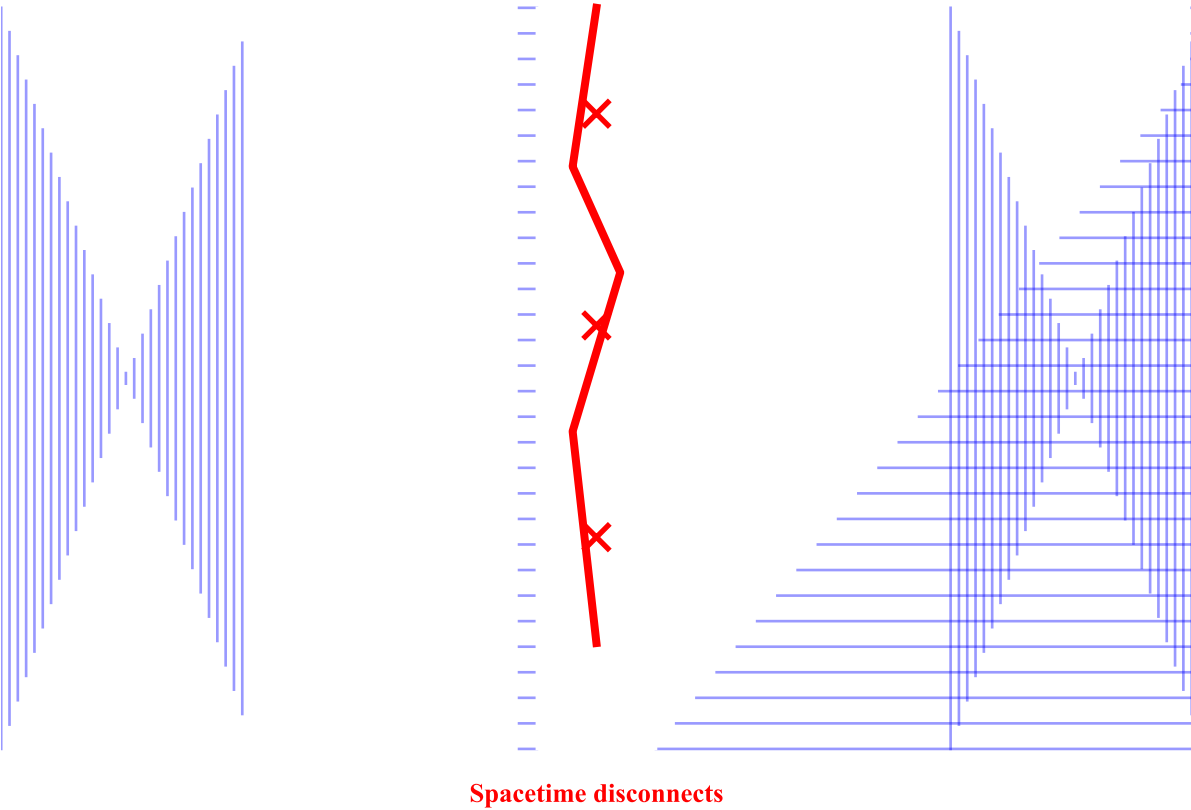
Cutting Entanglement → Spacetime Tear
