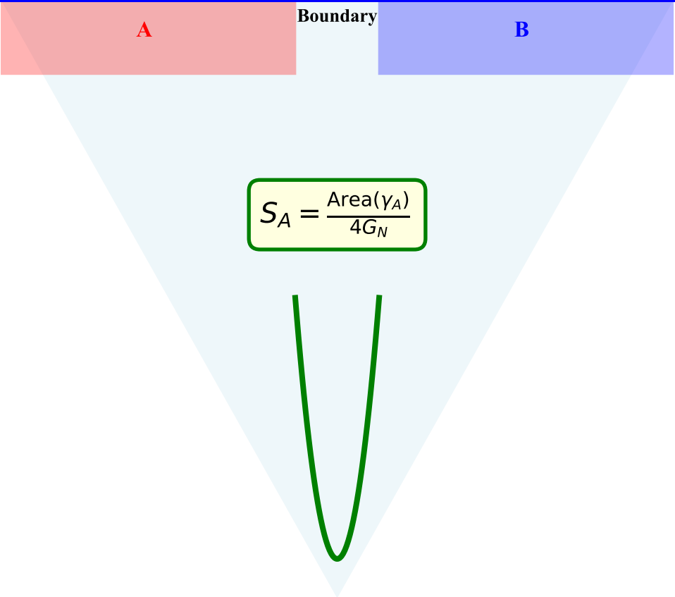
Ryu-Takayanagi: Entanglement = Minimal Surface
