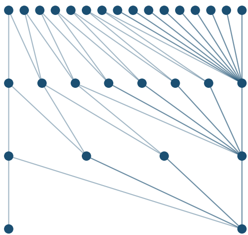
Tensor Network (MERA-like) Entanglement Pattern
