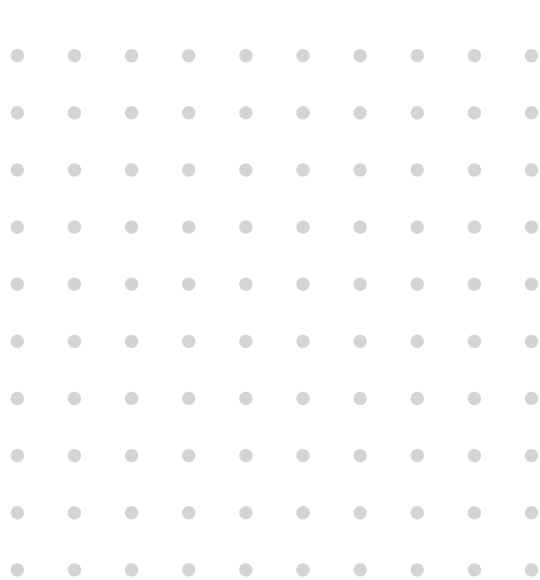
Uniform Modular Flow No Structure Remains
