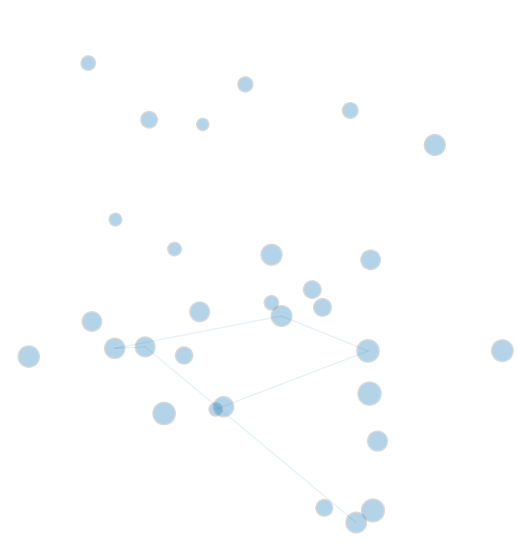
Sparse Correlations (Heat Death)
