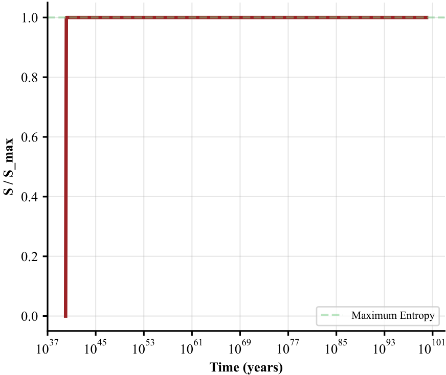
Entropy Saturation ( dS/dt \rightarrow 0 )
