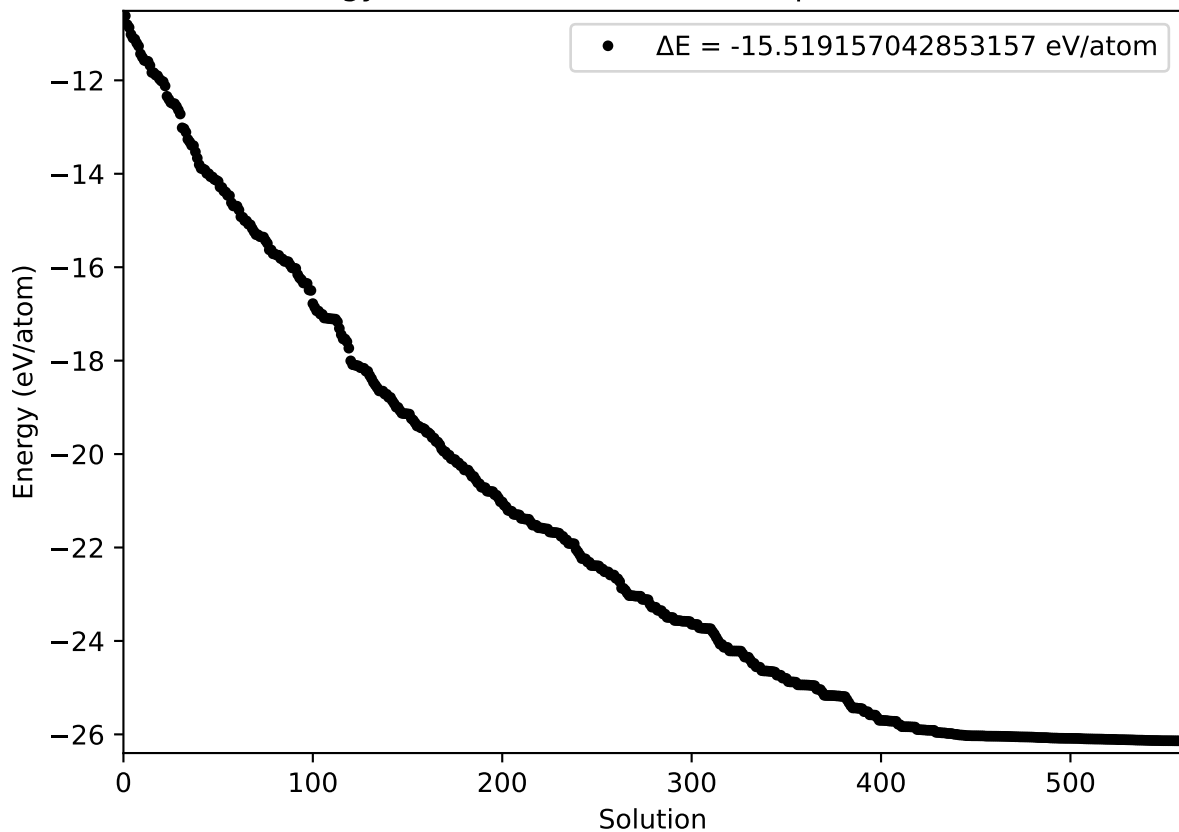
Energy of the best solutions sampled with SOSS
